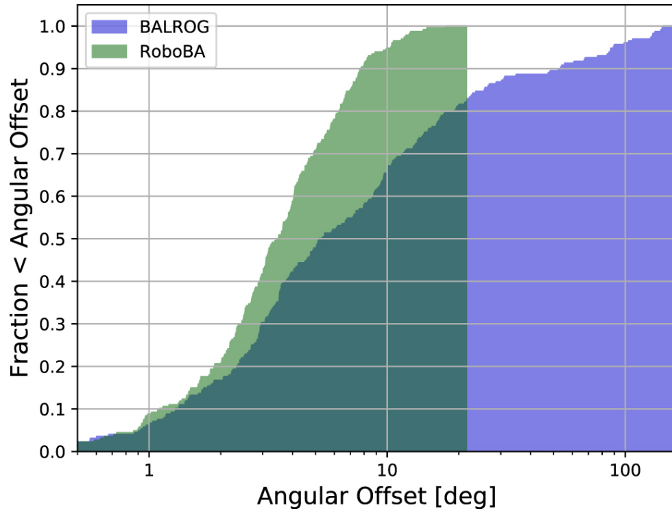
Figure 5. from Evaluation of Automated Fermi GBM Localizations of Gamma-Ray Bursts null 2020 APJ 895 40 doi:10.3847/1538-4357/ab8bdb https://dx.doi.org/10.3847/1538-4357/ab8bdb © 2020. The American Astronomical Society. All rights reserved.
