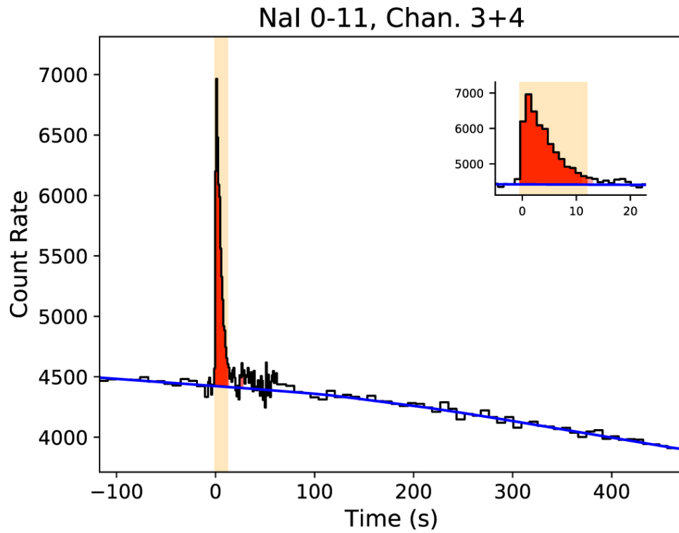
Figure 1. from Evaluation of Automated Fermi GBM Localizations of Gamma-Ray Bursts null 2020 APJ 895 40 doi:10.3847/1538-4357/ab8bdb https://dx.doi.org/10.3847/1538-4357/ab8bdb © 2020. The American Astronomical Society. All rights reserved.
