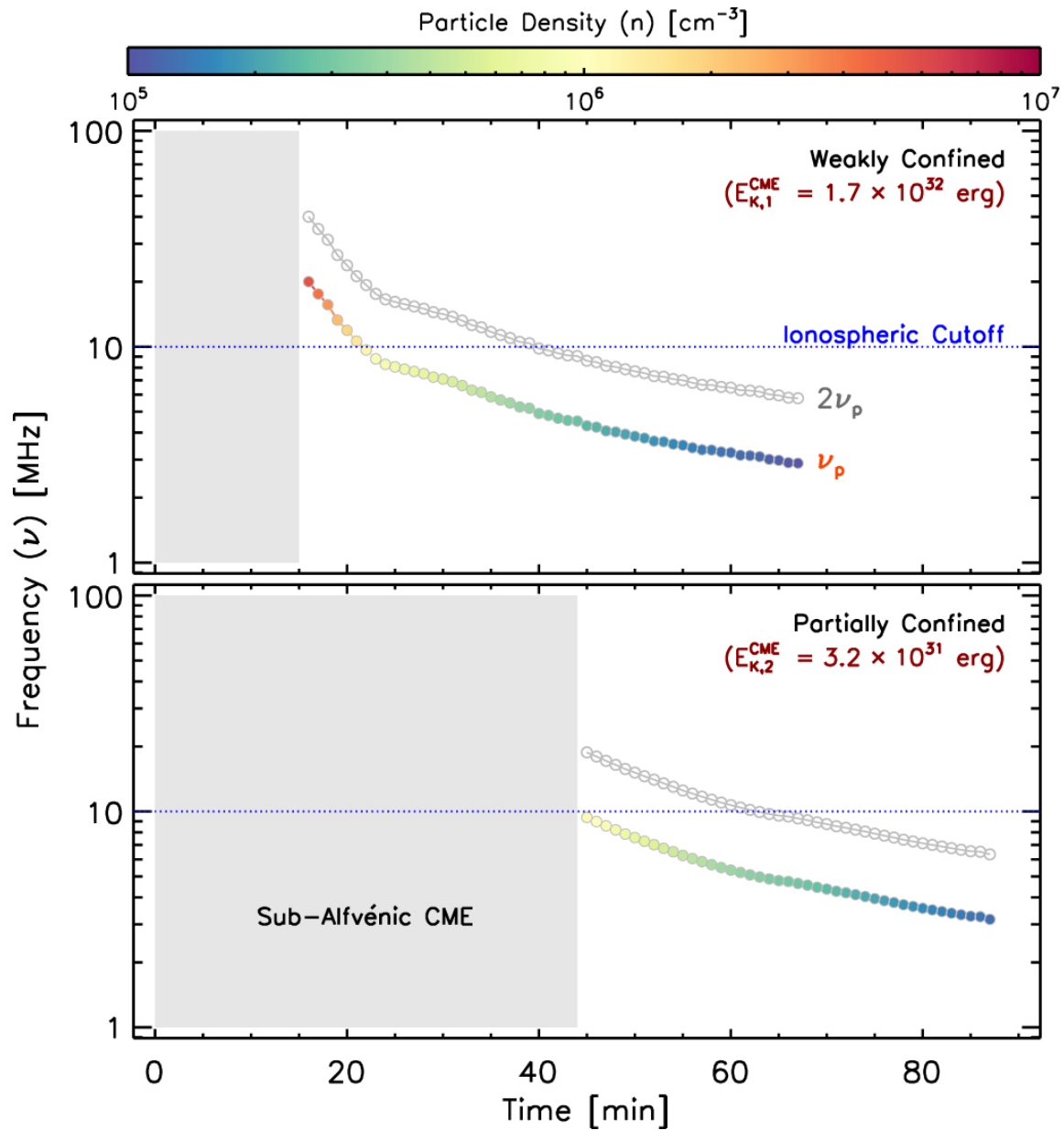
Figure 6. from Tuning the Exospace Weather Radio for Stellar Coronal Mass Ejections null 2020 APJ 895 47 doi:10.3847/1538-4357/ab88a3 https://dx.doi.org/10.3847/1538-4357/ab88a3 © 2020. The American Astronomical Society. All rights reserved.
