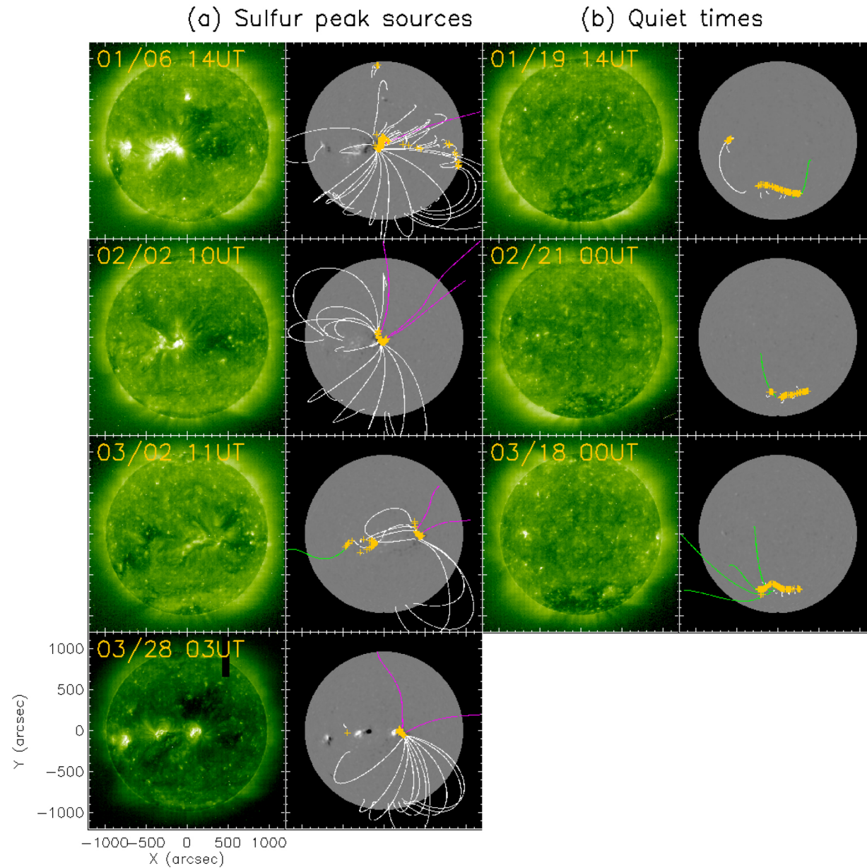
Figure 3. from Magnetic Field Geometry and Composition Variation in Slow Solar Winds: The Case of Sulfur null 2020 APJ 895 36 doi:10.3847/1538-4357/ab8870 https://dx.doi.org/10.3847/1538-4357/ab8870 © 2020. The American Astronomical Society. All rights reserved.
