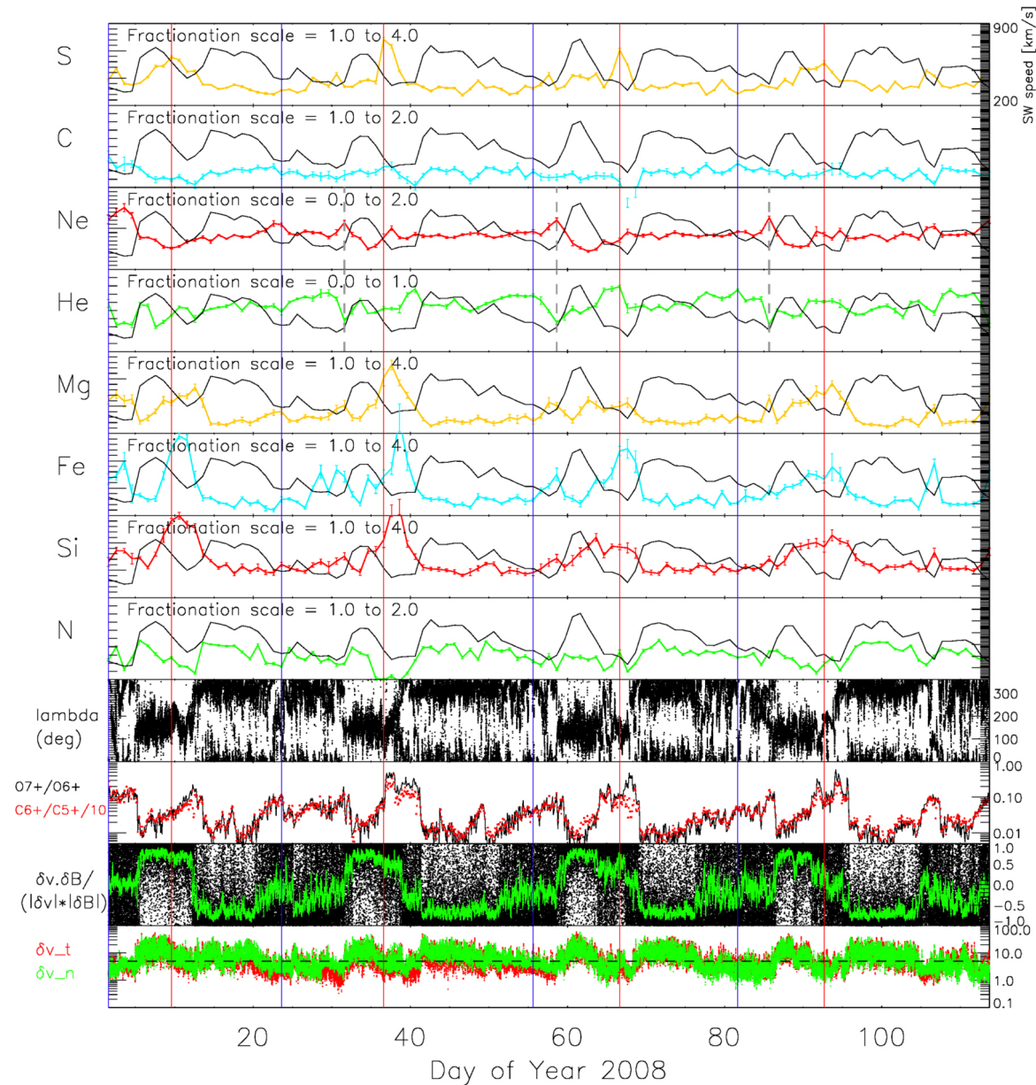
Figure 1. from Magnetic Field Geometry and Composition Variation in Slow Solar Winds: The Case of Sulfur null 2020 APJ 895 36 doi:10.3847/1538-4357/ab8870 https://dx.doi.org/10.3847/1538-4357/ab8870 © 2020. The American Astronomical Society. All rights reserved.
