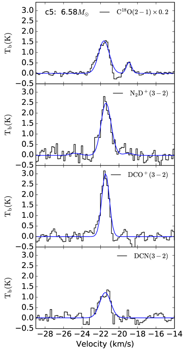
Figure 9. from Gas Kinematics of the Massive Protocluster G286.21+0.17 Revealed by ALMA null 2020 APJ 894 87 doi:10.3847/1538-4357/ab879f https://dx.doi.org/10.3847/1538-4357/ab879f © 2020. The American Astronomical Society. All rights reserved.
