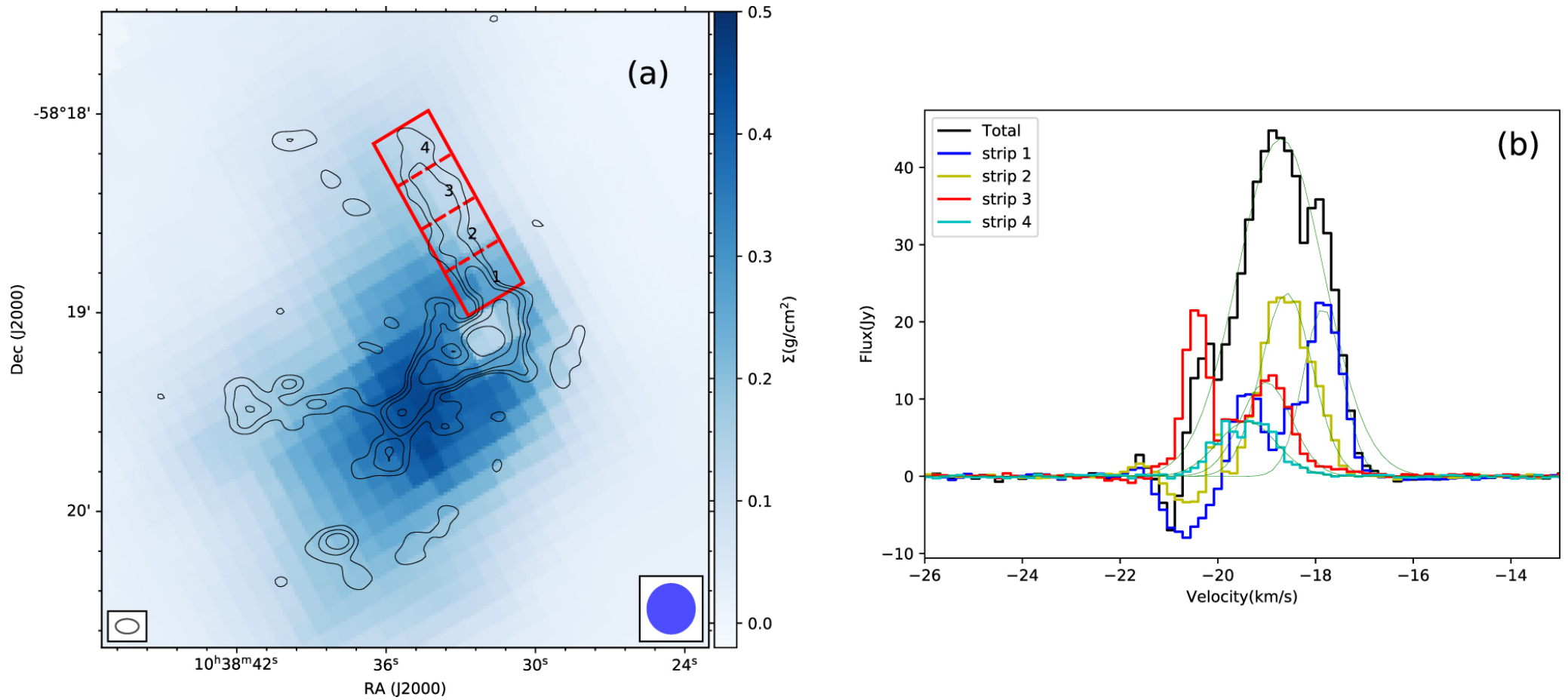
Figure 7. from Gas Kinematics of the Massive Protocluster G286.21+0.17 Revealed by ALMA null 2020 APJ 894 87 doi:10.3847/1538-4357/ab879f https://dx.doi.org/10.3847/1538-4357/ab879f © 2020. The American Astronomical Society. All rights reserved.
