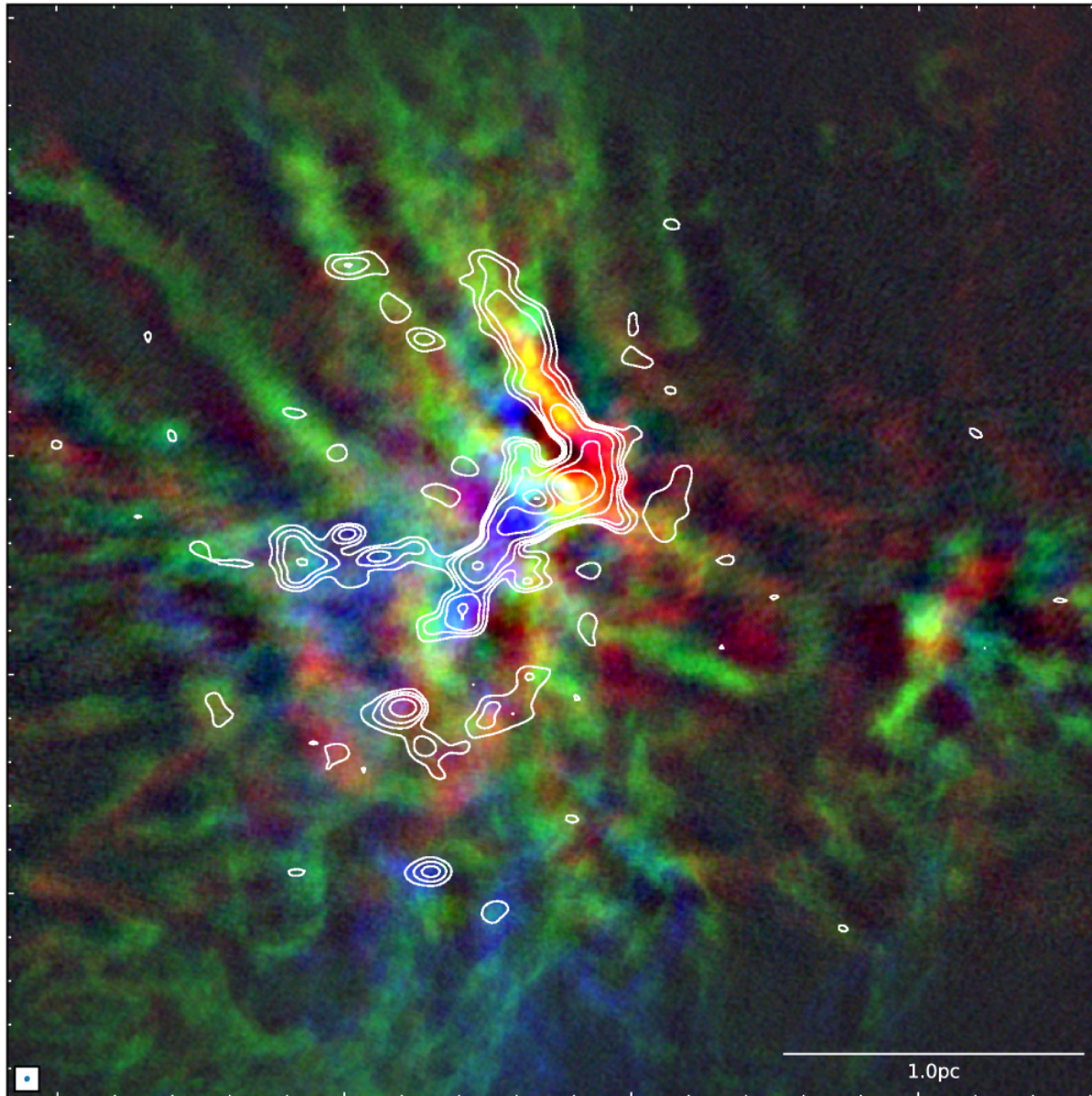
Figure 5. from Gas Kinematics of the Massive Protocluster G286.21+0.17 Revealed by ALMA null 2020 APJ 894 87 doi:10.3847/1538-4357/ab879f https://dx.doi.org/10.3847/1538-4357/ab879f © 2020. The American Astronomical Society. All rights reserved.
