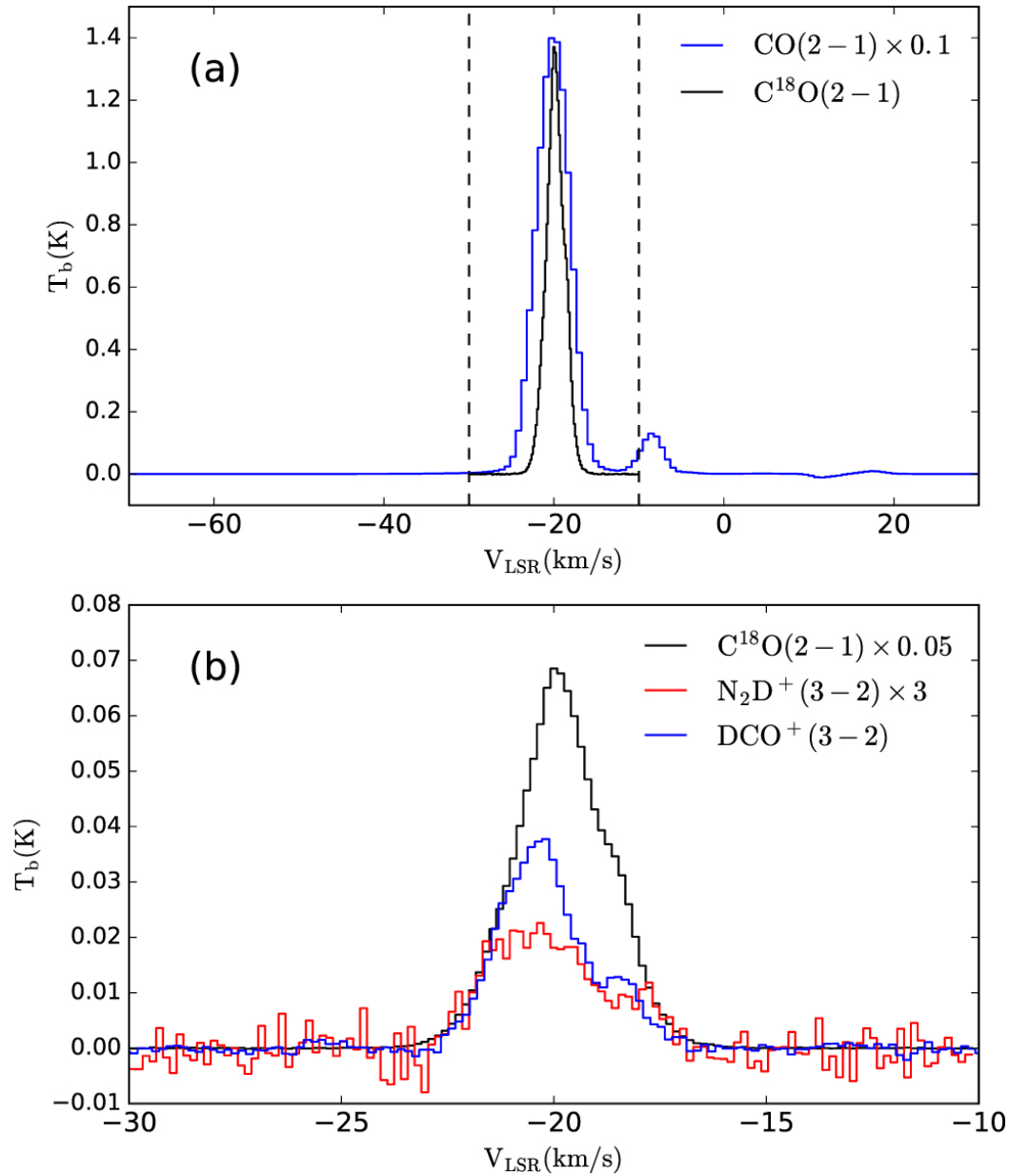
Figure 2. from Gas Kinematics of the Massive Protocluster G286.21+0.17 Revealed by ALMA null 2020 APJ 894 87 doi:10.3847/1538-4357/ab879f https://dx.doi.org/10.3847/1538-4357/ab879f © 2020. The American Astronomical Society. All rights reserved.
