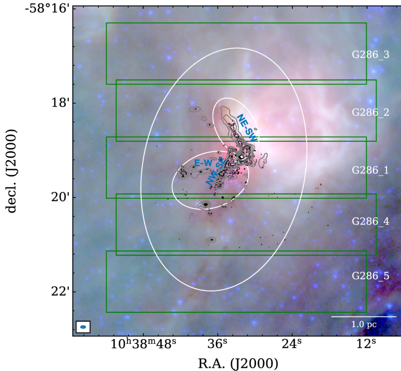
Figure 1. from Gas Kinematics of the Massive Protocluster G286.21+0.17 Revealed by ALMA null 2020 APJ 894 87 doi:10.3847/1538-4357/ab879f https://dx.doi.org/10.3847/1538-4357/ab879f © 2020. The American Astronomical Society. All rights reserved.
