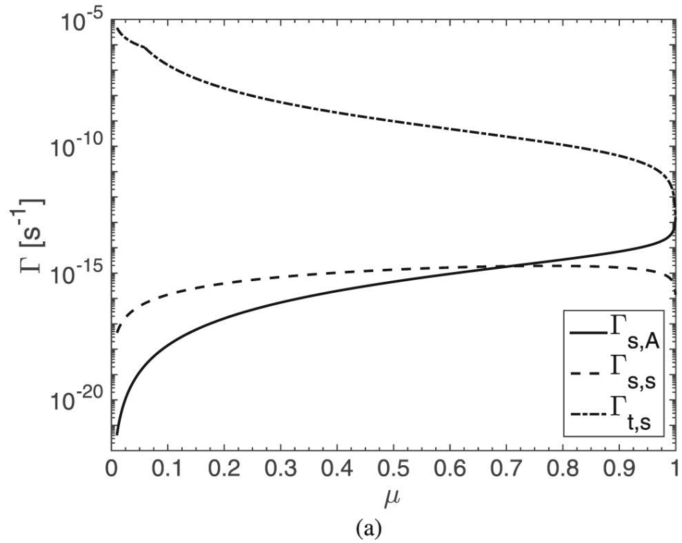
Figure 6. from Trapping of Cosmic Rays in MHD Turbulence null 2020 APJ 894 63 doi:10.3847/1538-4357/ab8465 https://dx.doi.org/10.3847/1538-4357/ab8465 © 2020. The American Astronomical Society. All rights reserved.
