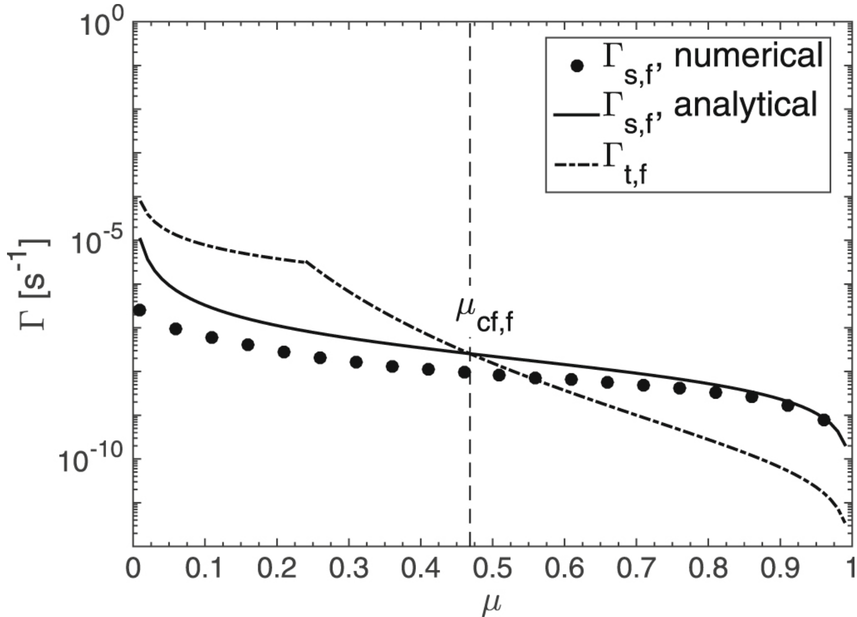
Figure 4. from Trapping of Cosmic Rays in MHD Turbulence null 2020 APJ 894 63 doi:10.3847/1538-4357/ab8465 https://dx.doi.org/10.3847/1538-4357/ab8465 © 2020. The American Astronomical Society. All rights reserved.
