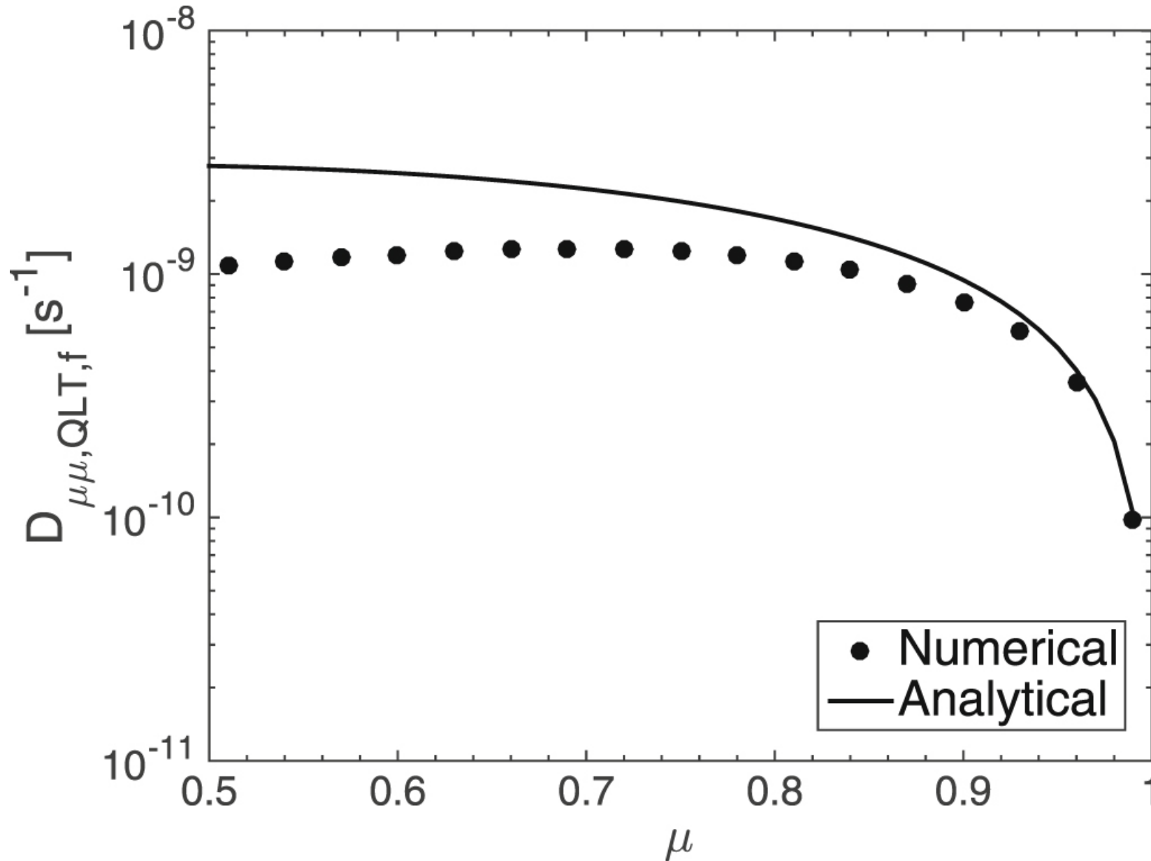
Figure 3. from Trapping of Cosmic Rays in MHD Turbulence null 2020 APJ 894 63 doi:10.3847/1538-4357/ab8465 https://dx.doi.org/10.3847/1538-4357/ab8465 © 2020. The American Astronomical Society. All rights reserved.
