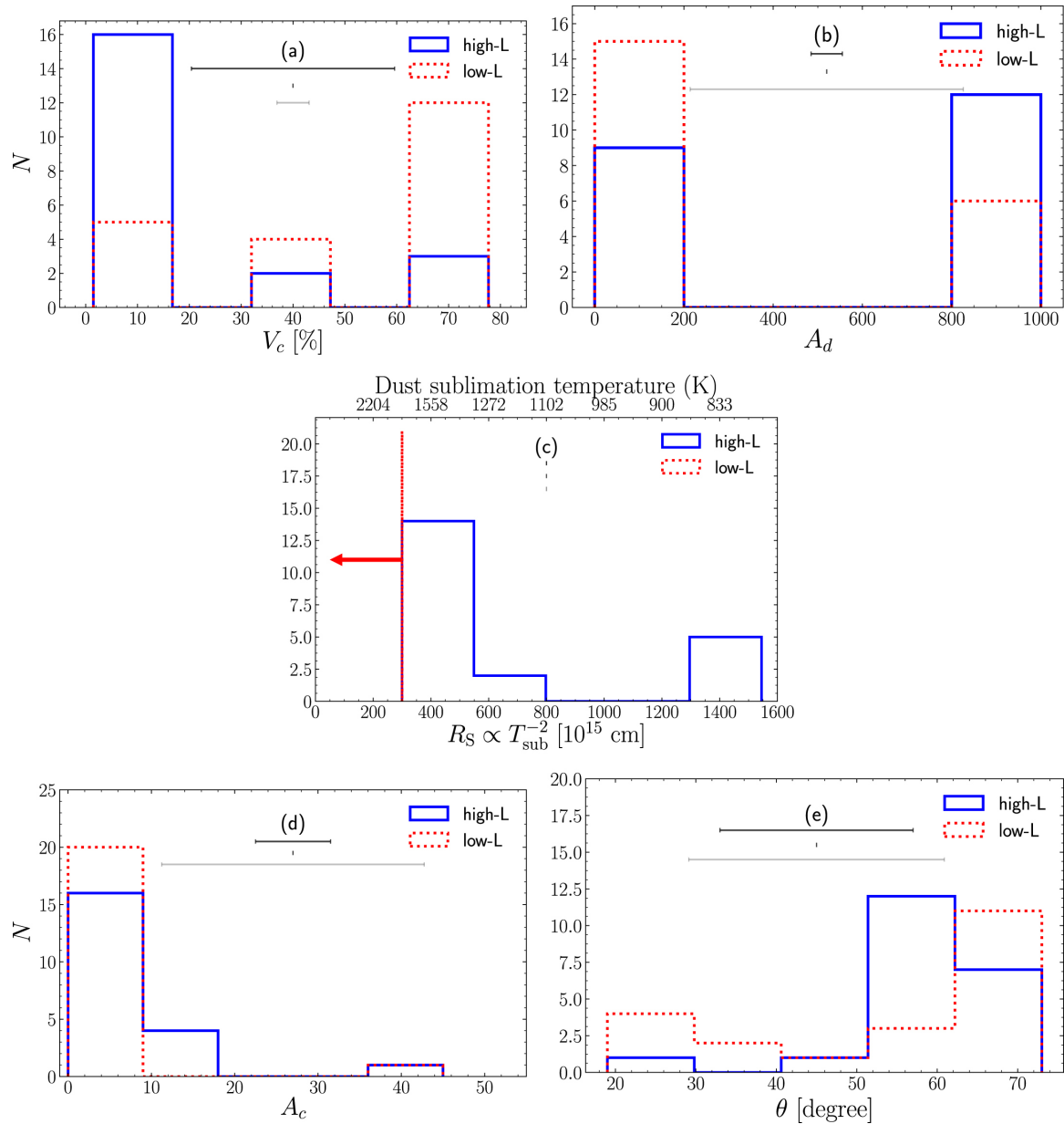
Figure 8. from AGNs Are Not That Cool: Revisiting the Intrinsic AGN Far-infrared Spectral Energy Distribution null 2020 APJ 894 21 doi:10.3847/1538-4357/ab811a https://dx.doi.org/10.3847/1538-4357/ab811a © 2020. The American Astronomical Society. All rights reserved.
