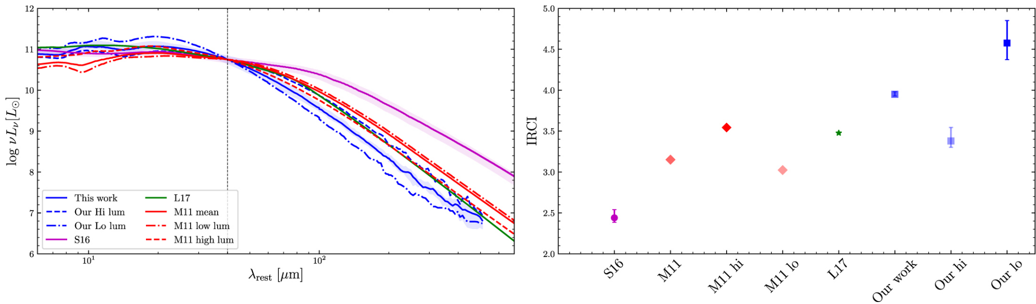
Figure 6. from AGNs Are Not That Cool: Revisiting the Intrinsic AGN Far-infrared Spectral Energy Distribution null 2020 APJ 894 21 doi:10.3847/1538-4357/ab811a https://dx.doi.org/10.3847/1538-4357/ab811a © 2020. The American Astronomical Society. All rights reserved.
