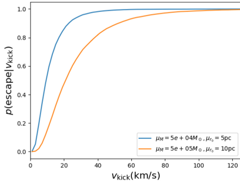
Figure 7. from Black Hole Coagulation: Modeling Hierarchical Mergers in Black Hole Populations null 2020 APJ 893 35 doi:10.3847/1538-4357/ab7fac https://dx.doi.org/10.3847/1538-4357/ab7fac © 2020. The American Astronomical Society. All rights reserved.
