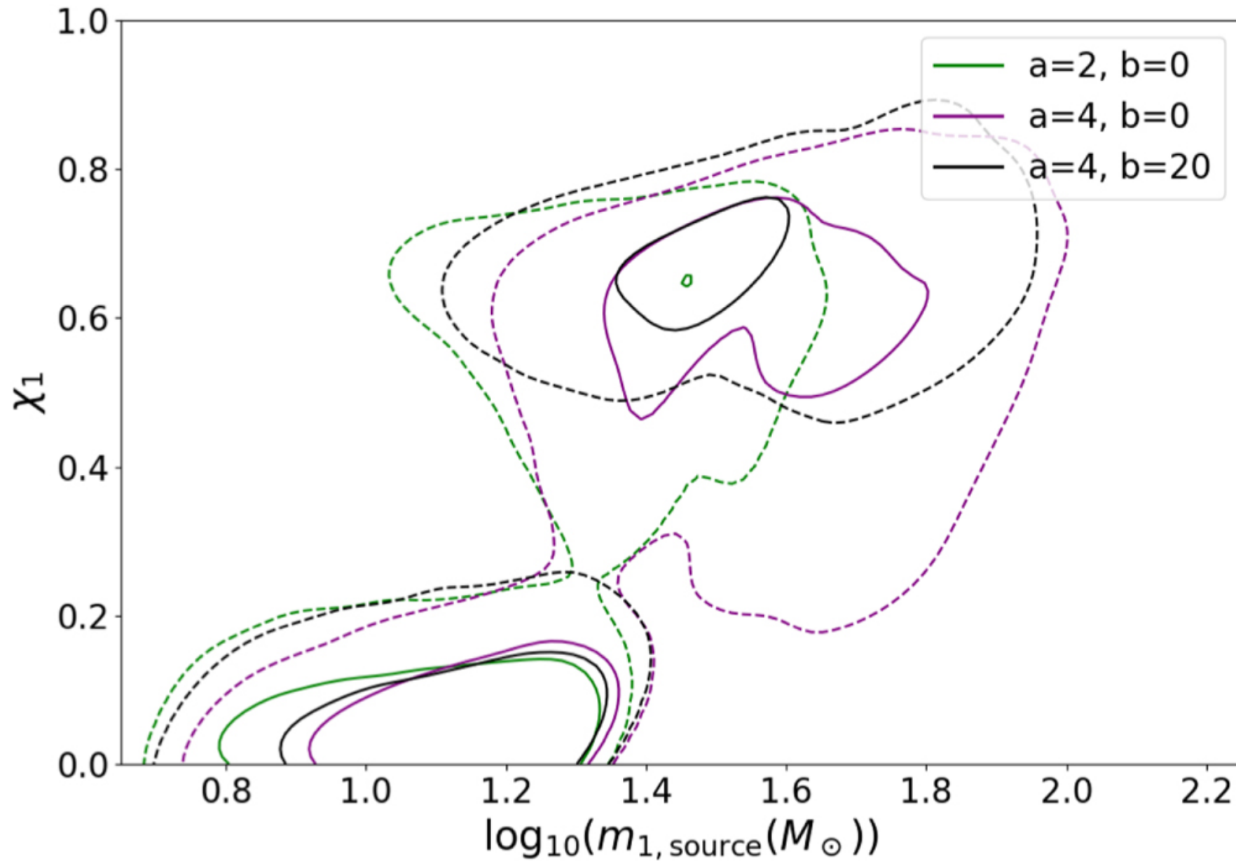
Figure 6. from Black Hole Coagulation: Modeling Hierarchical Mergers in Black Hole Populations null 2020 APJ 893 35 doi:10.3847/1538-4357/ab7fac https://dx.doi.org/10.3847/1538-4357/ab7fac © 2020. The American Astronomical Society. All rights reserved.
