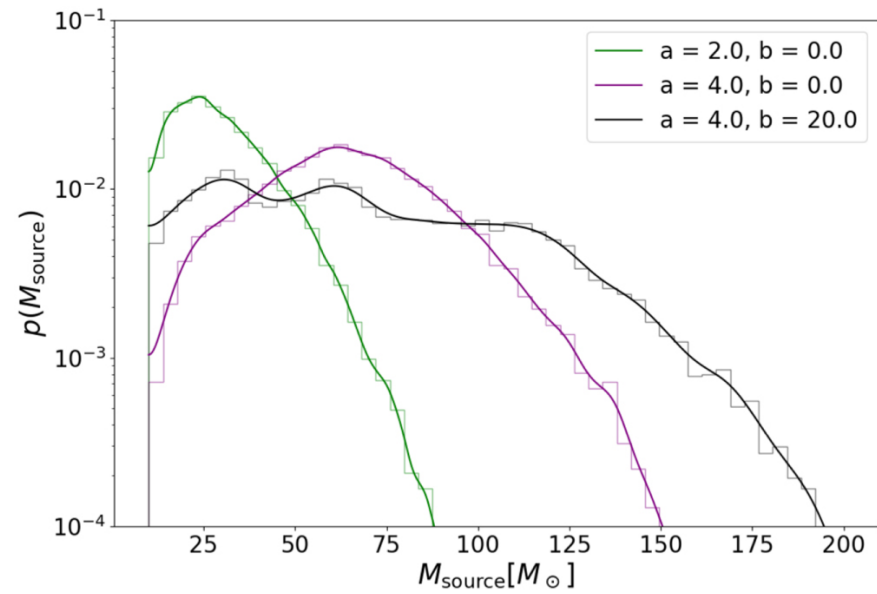
Figure 4. from Black Hole Coagulation: Modeling Hierarchical Mergers in Black Hole Populations null 2020 APJ 893 35 doi:10.3847/1538-4357/ab7fac https://dx.doi.org/10.3847/1538-4357/ab7fac
