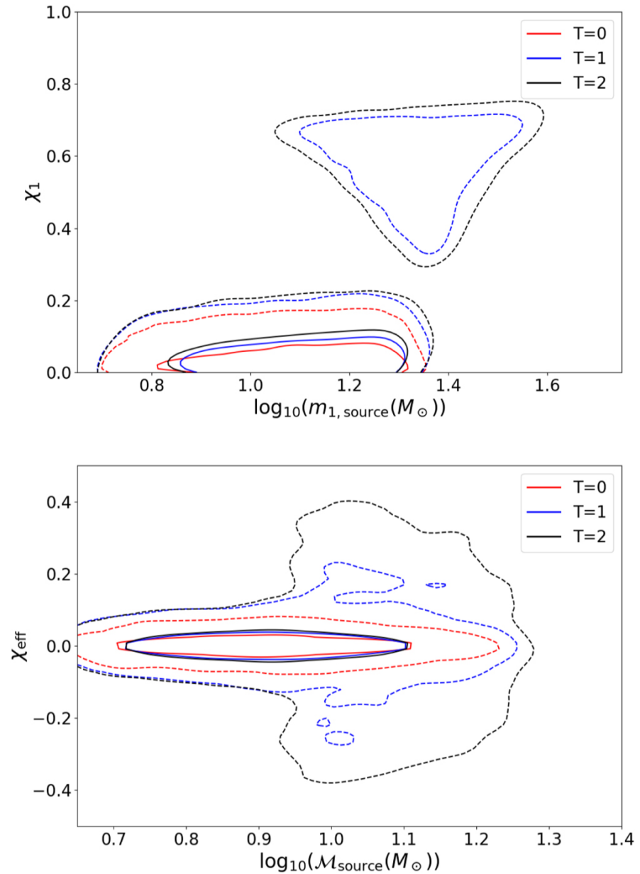
Figure 3. from Black Hole Coagulation: Modeling Hierarchical Mergers in Black Hole Populations null 2020 APJ 893 35 doi:10.3847/1538-4357/ab7fac https://dx.doi.org/10.3847/1538-4357/ab7fac © 2020. The American Astronomical Society. All rights reserved.
