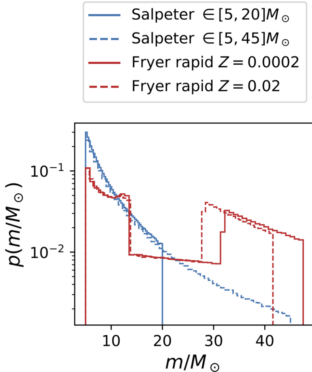
Figure 1. from Black Hole Coagulation: Modeling Hierarchical Mergers in Black Hole Populations null 2020 APJ 893 35 doi:10.3847/1538-4357/ab7fac https://dx.doi.org/10.3847/1538-4357/ab7fac © 2020. The American Astronomical Society. All rights reserved.
