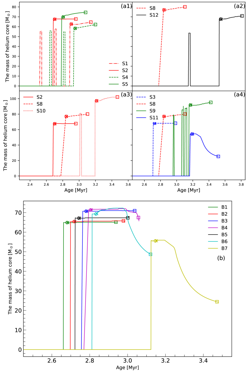
Figure 10. from The Structure and Evolution of Massive Rotating Single and Binary Population III Stars null 2020 APJ 892 41 doi:10.3847/1538-4357/ab7993 https://dx.doi.org/10.3847/1538-4357/ab7993 © 2020. The American Astronomical Society. All rights reserved.
