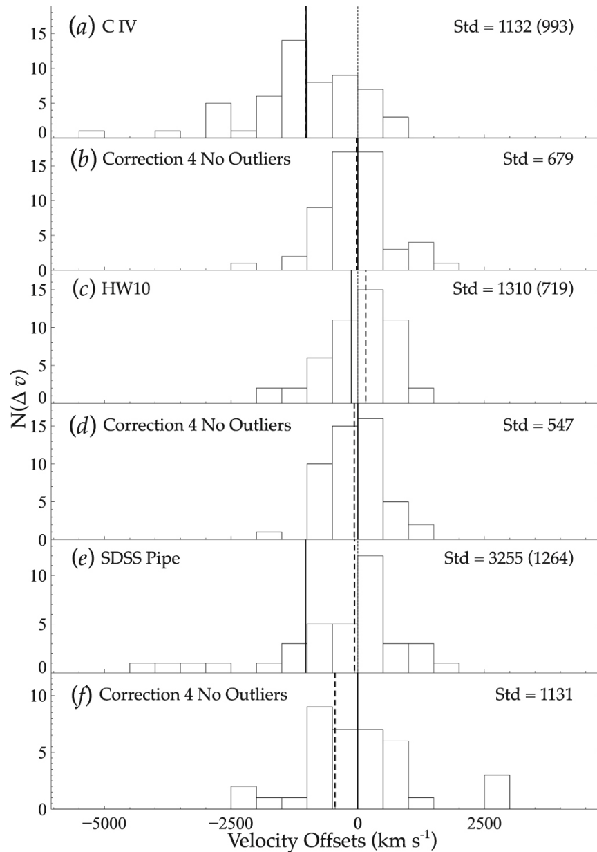
Figure 5. from Prescriptions for Correcting Ultraviolet-based Redshifts for Luminous Quasars at High Redshift null 2020 APJ 893 14 doi:10.3847/1538-4357/ab77b6 https://dx.doi.org/10.3847/1538-4357/ab77b6 © 2020. The American Astronomical Society. All rights reserved.
