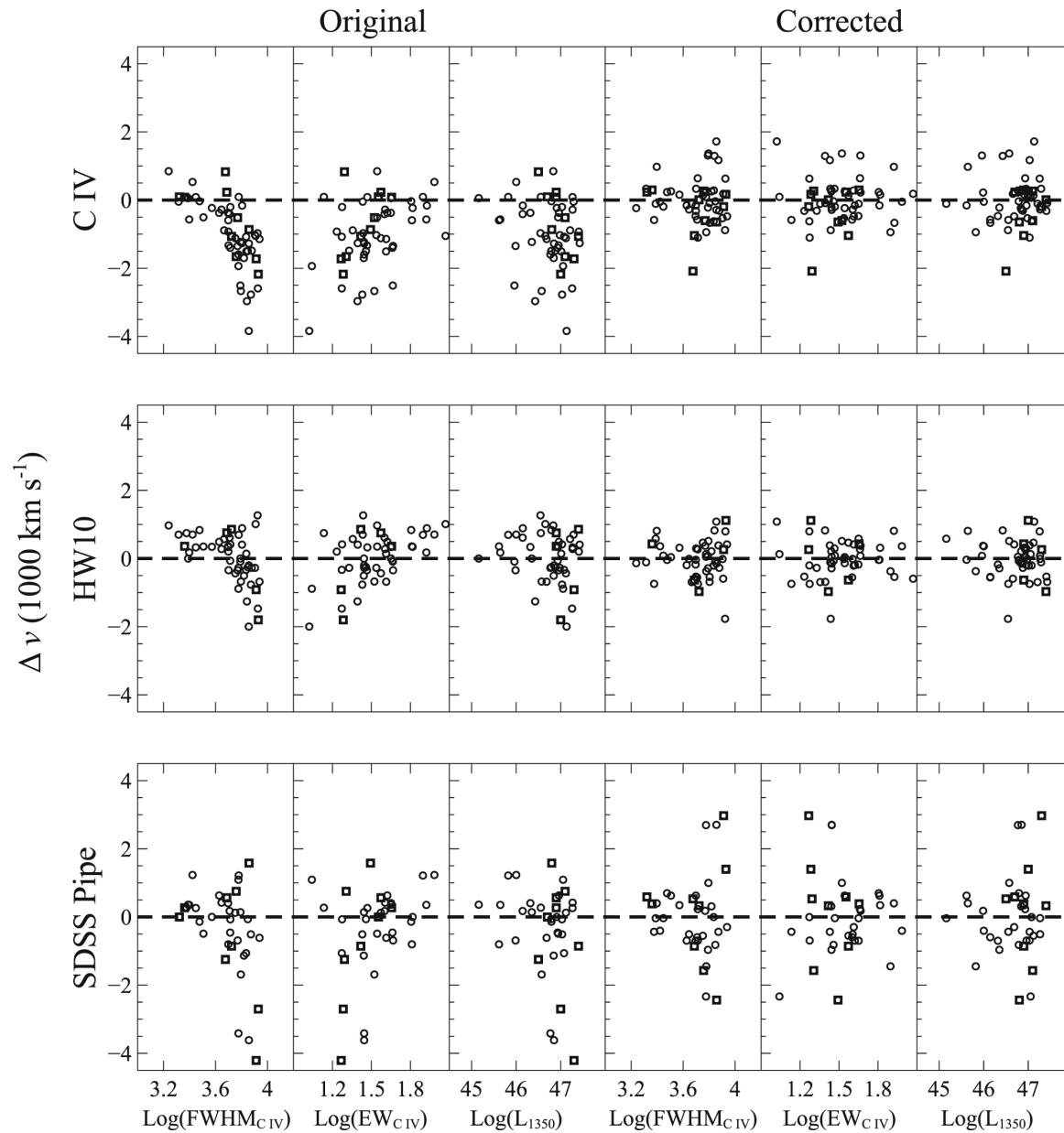
Figure 4. from Prescriptions for Correcting Ultraviolet-based Redshifts for Luminous Quasars at High Redshift null 2020 APJ 893 14 doi:10.3847/1538-4357/ab77b6 https://dx.doi.org/10.3847/1538-4357/ab77b6 © 2020. The American Astronomical Society. All rights reserved.
