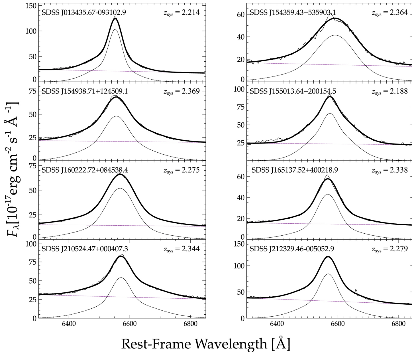
Figure 2. from Prescriptions for Correcting Ultraviolet-based Redshifts for Luminous Quasars at High Redshift null 2020 APJ 893 14 doi:10.3847/1538-4357/ab77b6 https://dx.doi.org/10.3847/1538-4357/ab77b6 © 2020. The American Astronomical Society. All rights reserved.
