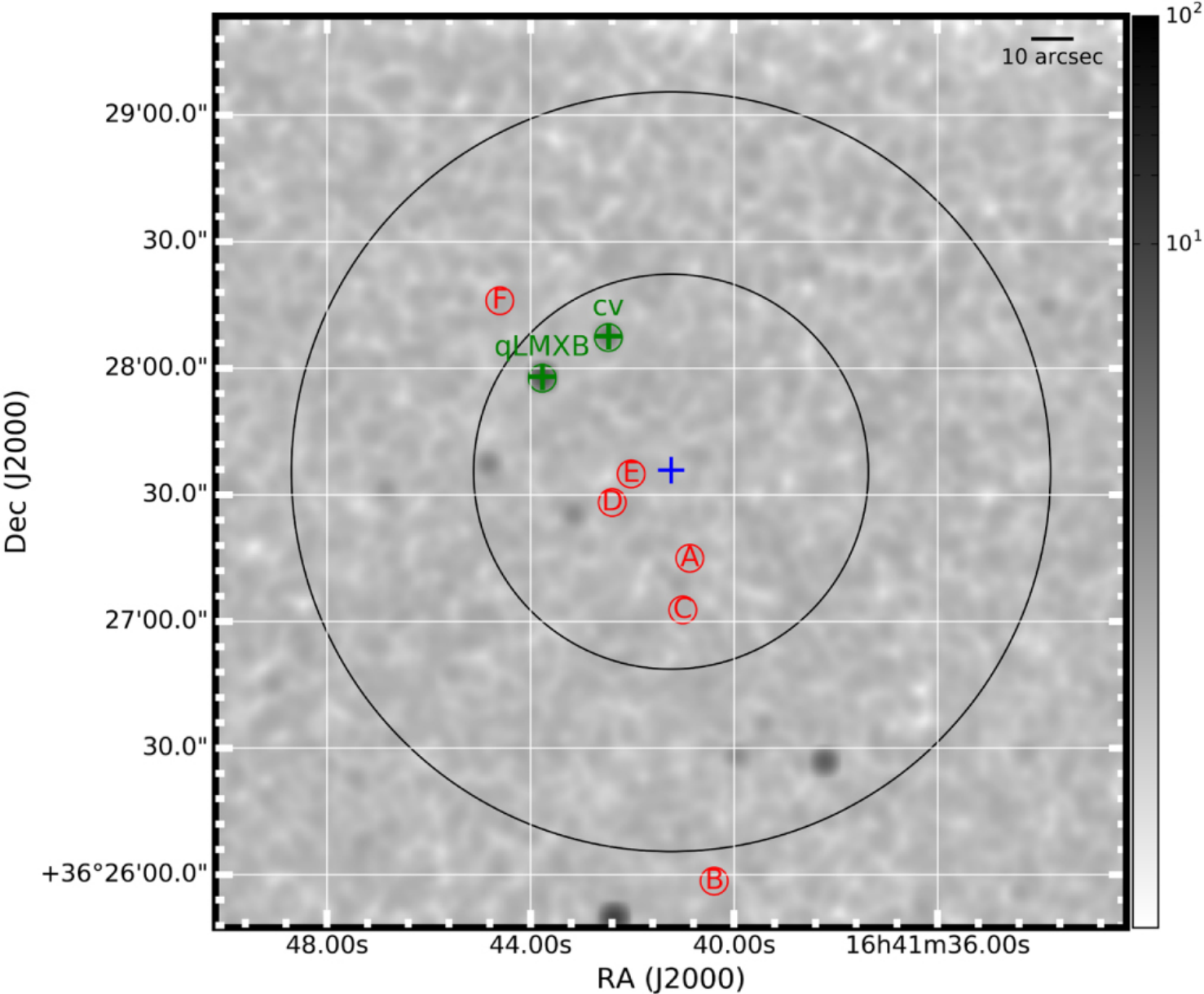
Figure 6. from Discovery and Timing of Pulsars in the Globular Cluster M13 with FAST null 2020 APJ 892 43 doi:10.3847/1538-4357/ab76cc https://dx.doi.org/10.3847/1538-4357/ab76cc © 2020. The American Astronomical Society. All rights reserved.
