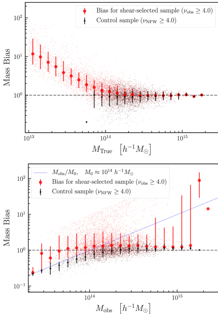
Figure 6. from Mass Bias of Weak-lensing Shear-selected Galaxy Cluster Samples null 2020 APJ 891 139 doi:10.3847/1538-4357/ab74d3 https://dx.doi.org/10.3847/1538-4357/ab74d3 © 2020. The American Astronomical Society. All rights reserved.
