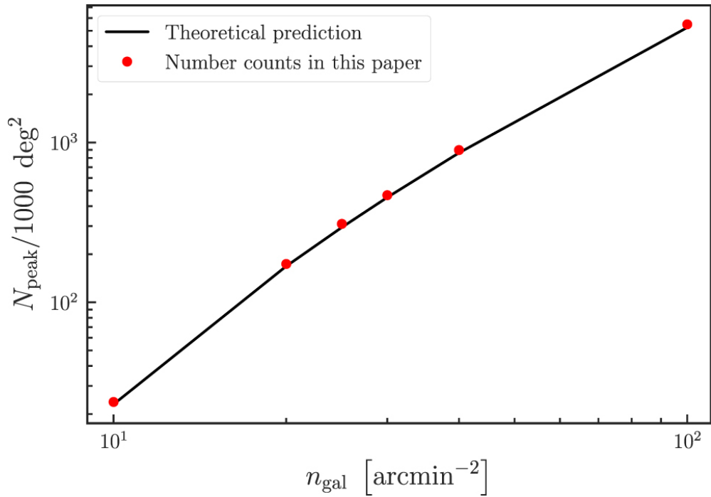
Figure 3. from Mass Bias of Weak-lensing Shear-selected Galaxy Cluster Samples null 2020 APJ 891 139 doi:10.3847/1538-4357/ab74d3 https://dx.doi.org/10.3847/1538-4357/ab74d3 © 2020. The American Astronomical Society. All rights reserved.
