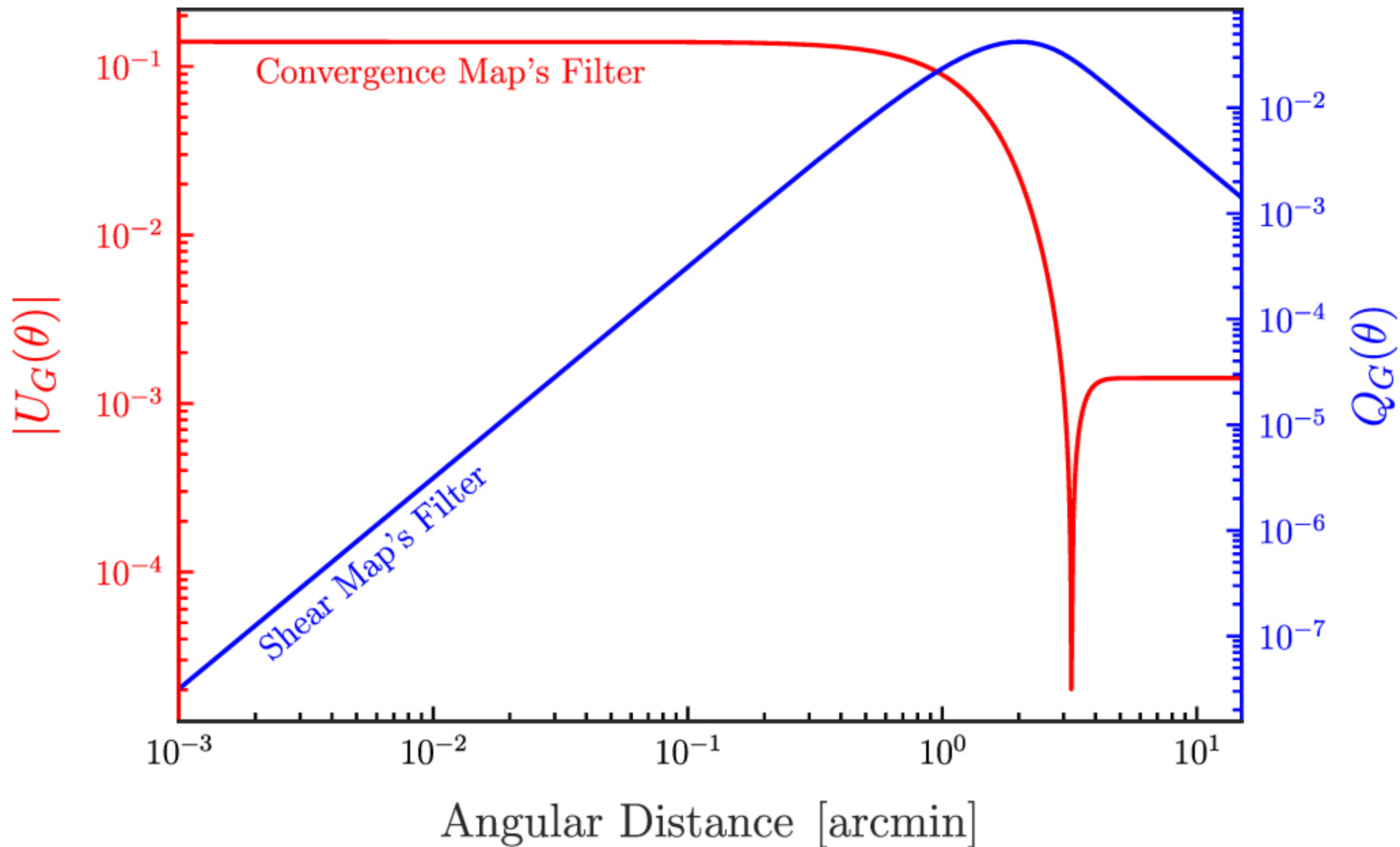
Figure 2. from Mass Bias of Weak-lensing Shear-selected Galaxy Cluster Samples null 2020 APJ 891 139 doi:10.3847/1538-4357/ab74d3 https://dx.doi.org/10.3847/1538-4357/ab74d3 © 2020. The American Astronomical Society. All rights reserved.
