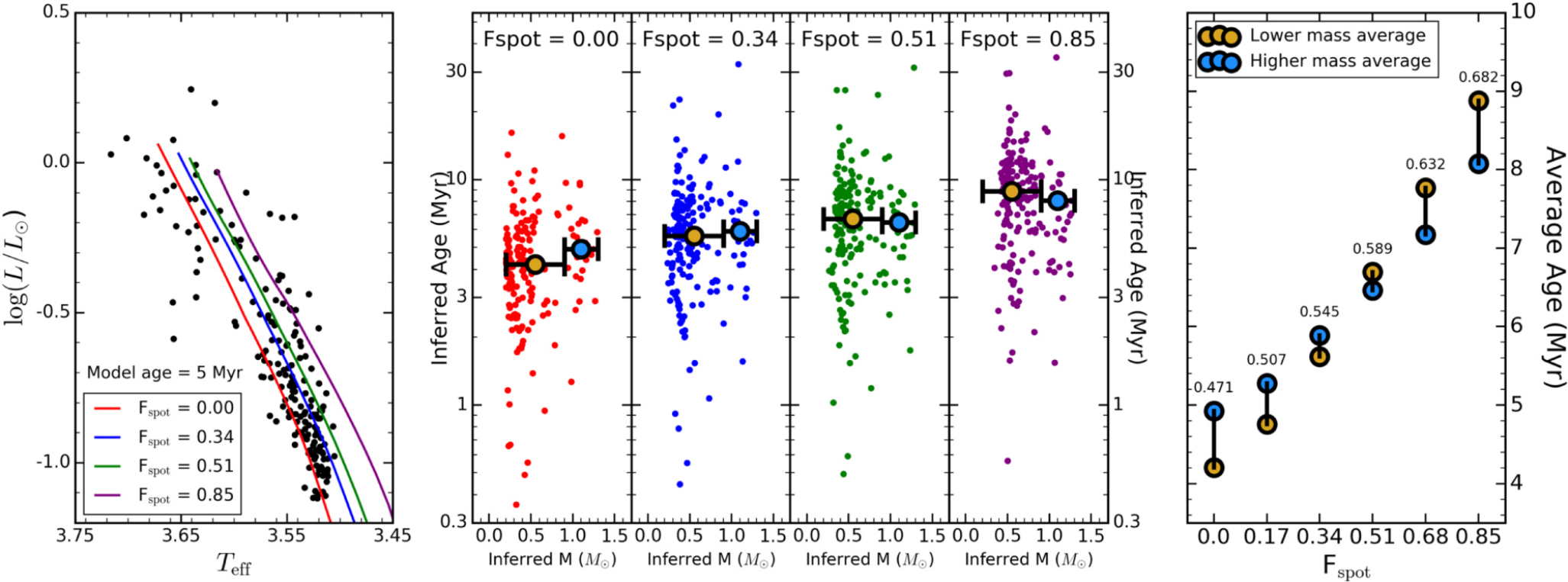
Figure 7. from The SPOTS Models: A Grid of Theoretical Stellar Evolution Tracks and Isochrones for Testing the Effects of Starspots on Structure and Colors null 2020 APJ 891 29 doi:10.3847/1538-4357/ab722e https://dx.doi.org/10.3847/1538-4357/ab722e © 2020. The American Astronomical Society. All rights reserved.
