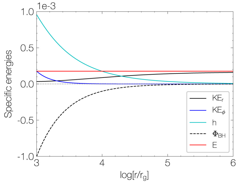
Figure 5. from Large-scale Dynamics of Winds Originating from Black Hole Accretion Flows. I. Hydrodynamics null 2020 APJ 890 80 doi:10.3847/1538-4357/ab6e6e https://dx.doi.org/10.3847/1538-4357/ab6e6e
