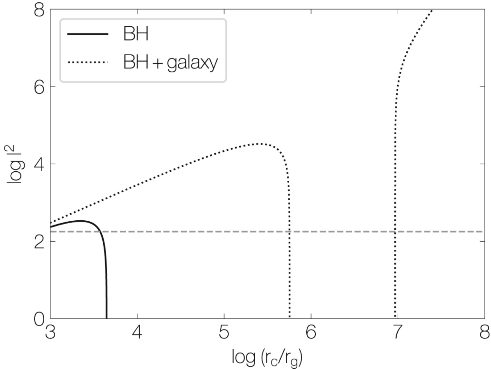
Figure 2. from Large-scale Dynamics of Winds Originating from Black Hole Accretion Flows. I. Hydrodynamics null 2020 APJ 890 80 doi:10.3847/1538-4357/ab6e6e https://dx.doi.org/10.3847/1538-4357/ab6e6e © 2020. The American Astronomical Society. All rights reserved.
