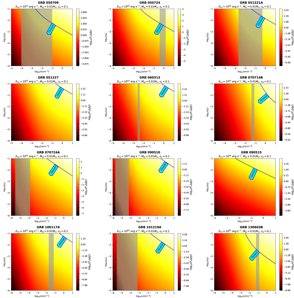
Figure 6. from Constraining the Long-lived Magnetar Remnants in Short Gamma-Ray Bursts from Late-time Radio Observations null 2020 APJ 890 102 doi:10.3847/1538-4357/ab6b24 https://dx.doi.org/10.3847/1538-4357/ab6b24
