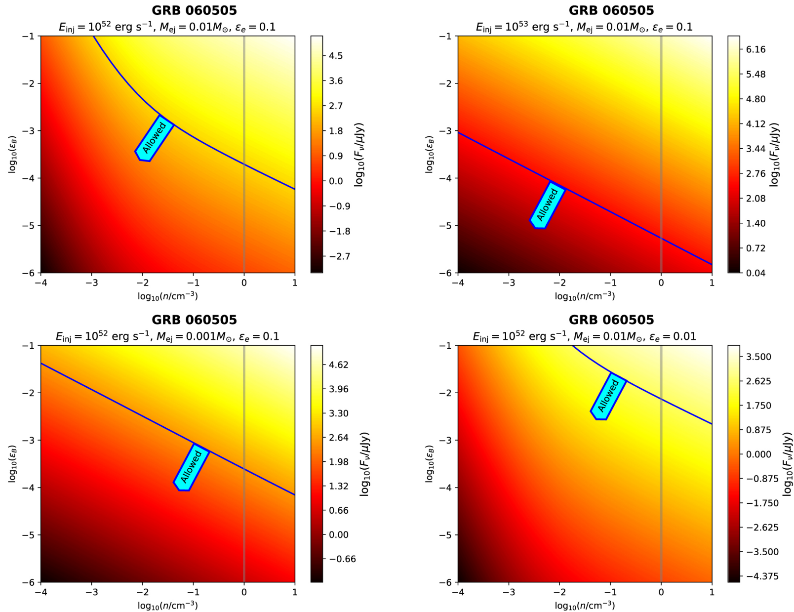
Figure 4. from Constraining the Long-lived Magnetar Remnants in Short Gamma-Ray Bursts from Late-time Radio Observations null 2020 APJ 890 102 doi:10.3847/1538-4357/ab6b24 https://dx.doi.org/10.3847/1538-4357/ab6b24 © 2020. The American Astronomical Society. All rights reserved.
