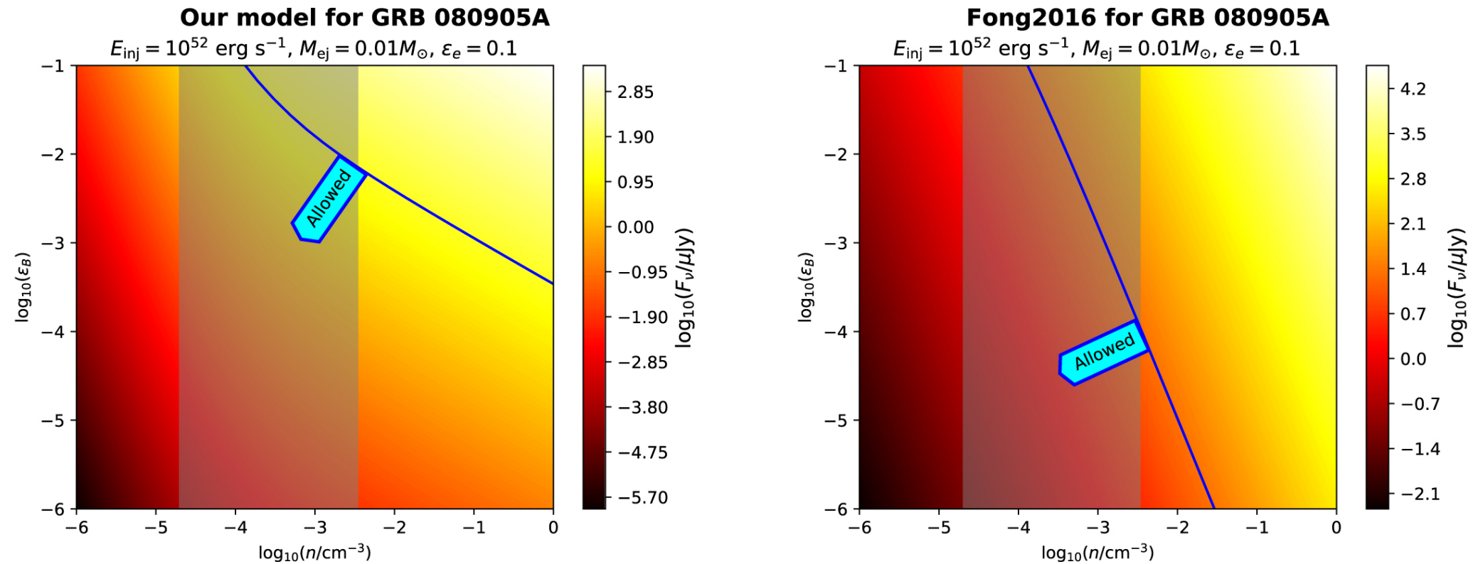
Figure 3. from Constraining the Long-lived Magnetar Remnants in Short Gamma-Ray Bursts from Late-time Radio Observations null 2020 APJ 890 102 doi:10.3847/1538-4357/ab6b24 https://dx.doi.org/10.3847/1538-4357/ab6b24 © 2020. The American Astronomical Society. All rights reserved.
