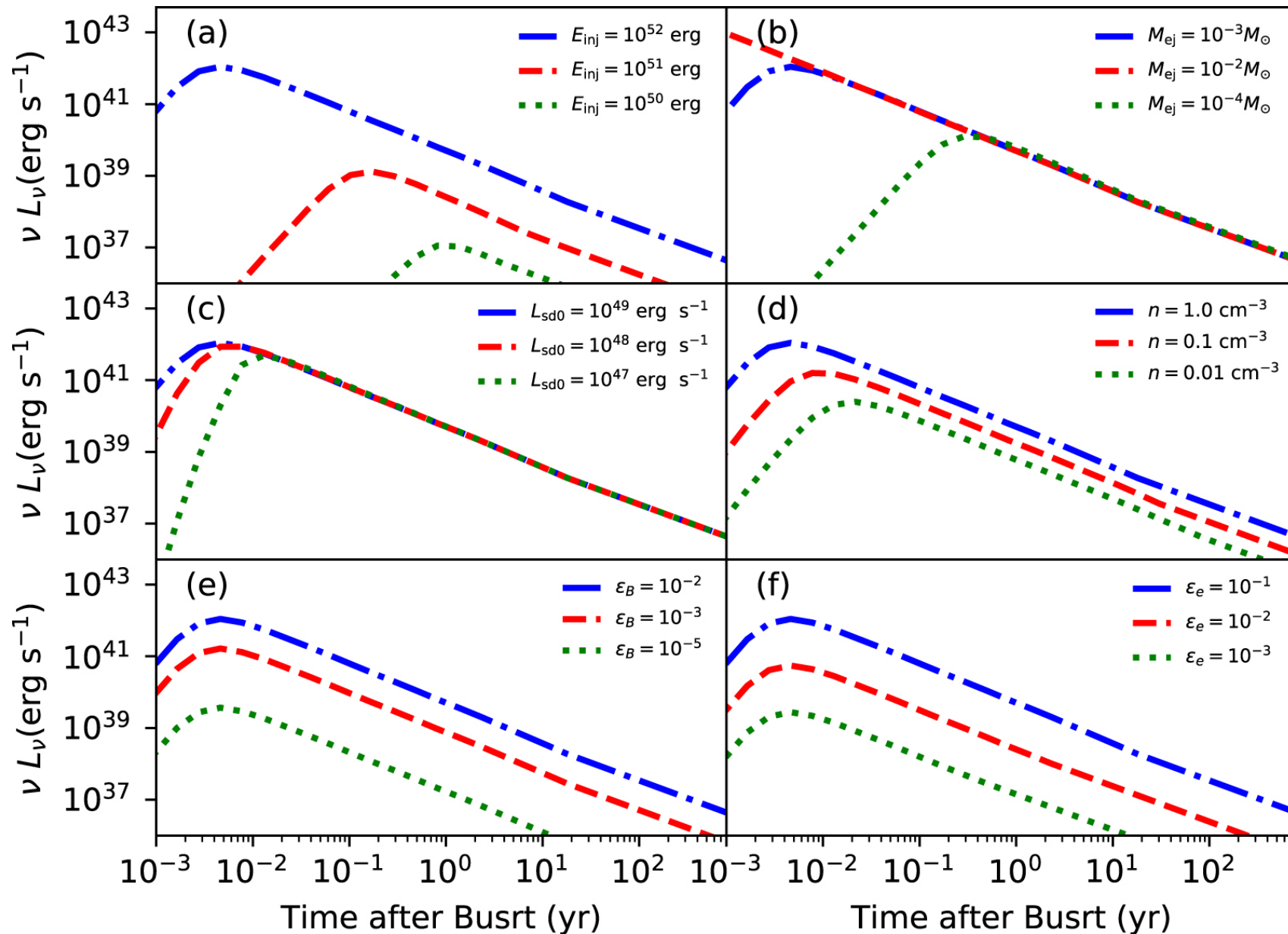
Figure 2. from Constraining the Long-lived Magnetar Remnants in Short Gamma-Ray Bursts from Late-time Radio Observations null 2020 APJ 890 102 doi:10.3847/1538-4357/ab6b24 https://dx.doi.org/10.3847/1538-4357/ab6b24 © 2020. The American Astronomical Society. All rights reserved.
