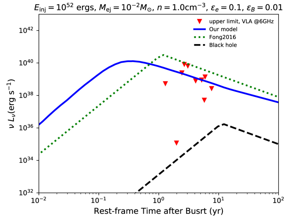
Figure 1. from Constraining the Long-lived Magnetar Remnants in Short Gamma-Ray Bursts from Late-time Radio Observations null 2020 APJ 890 102 doi:10.3847/1538-4357/ab6b24 https://dx.doi.org/10.3847/1538-4357/ab6b24
