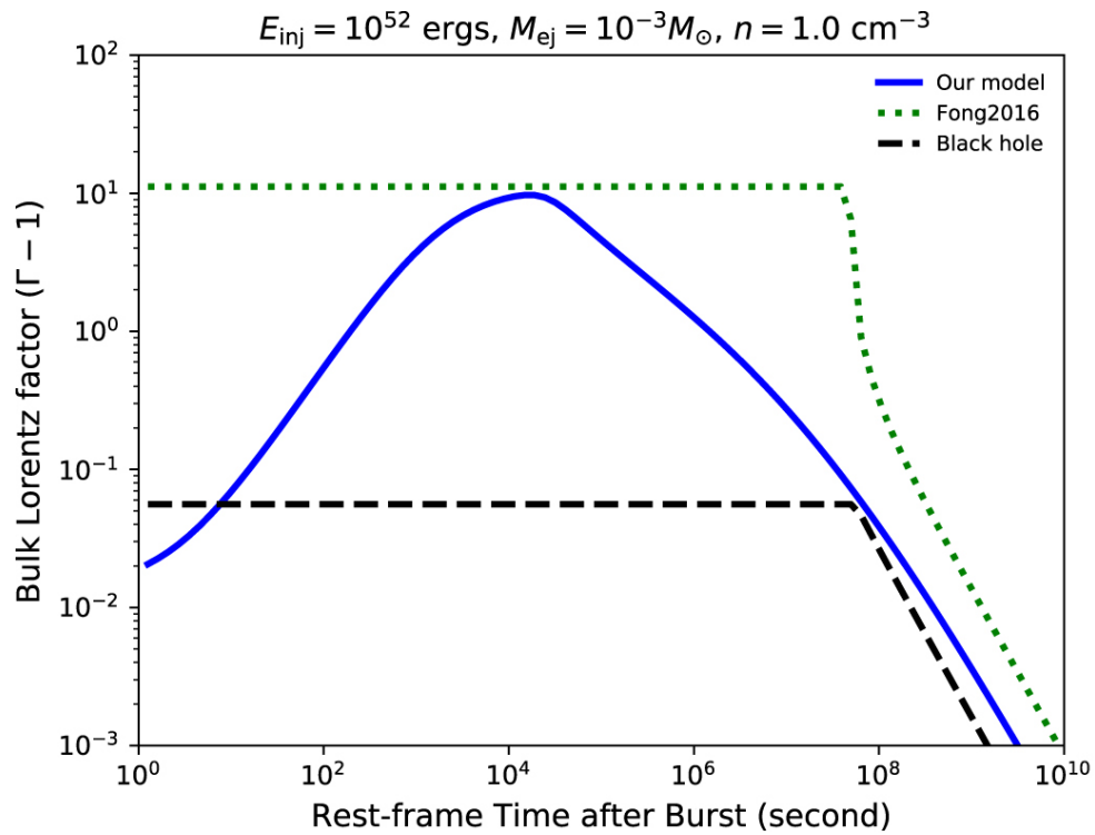
Figure 1. from Constraining the Long-lived Magnetar Remnants in Short Gamma-Ray Bursts from Late-time Radio Observations null 2020 APJ 890 102 doi:10.3847/1538-4357/ab6b24 https://dx.doi.org/10.3847/1538-4357/ab6b24
