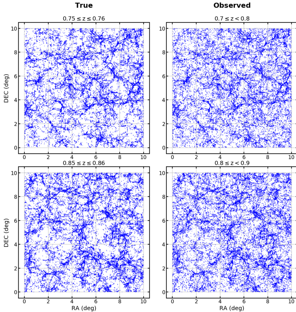
Figure 2. from Angular Correlation Function Estimators Accounting for Contamination from Probabilistic Distance Measurements null 2020 APJ 890 78 doi:10.3847/1538-4357/ab63c8 https://dx.doi.org/10.3847/1538-4357/ab63c8 © 2020. The American Astronomical Society. All rights reserved.
