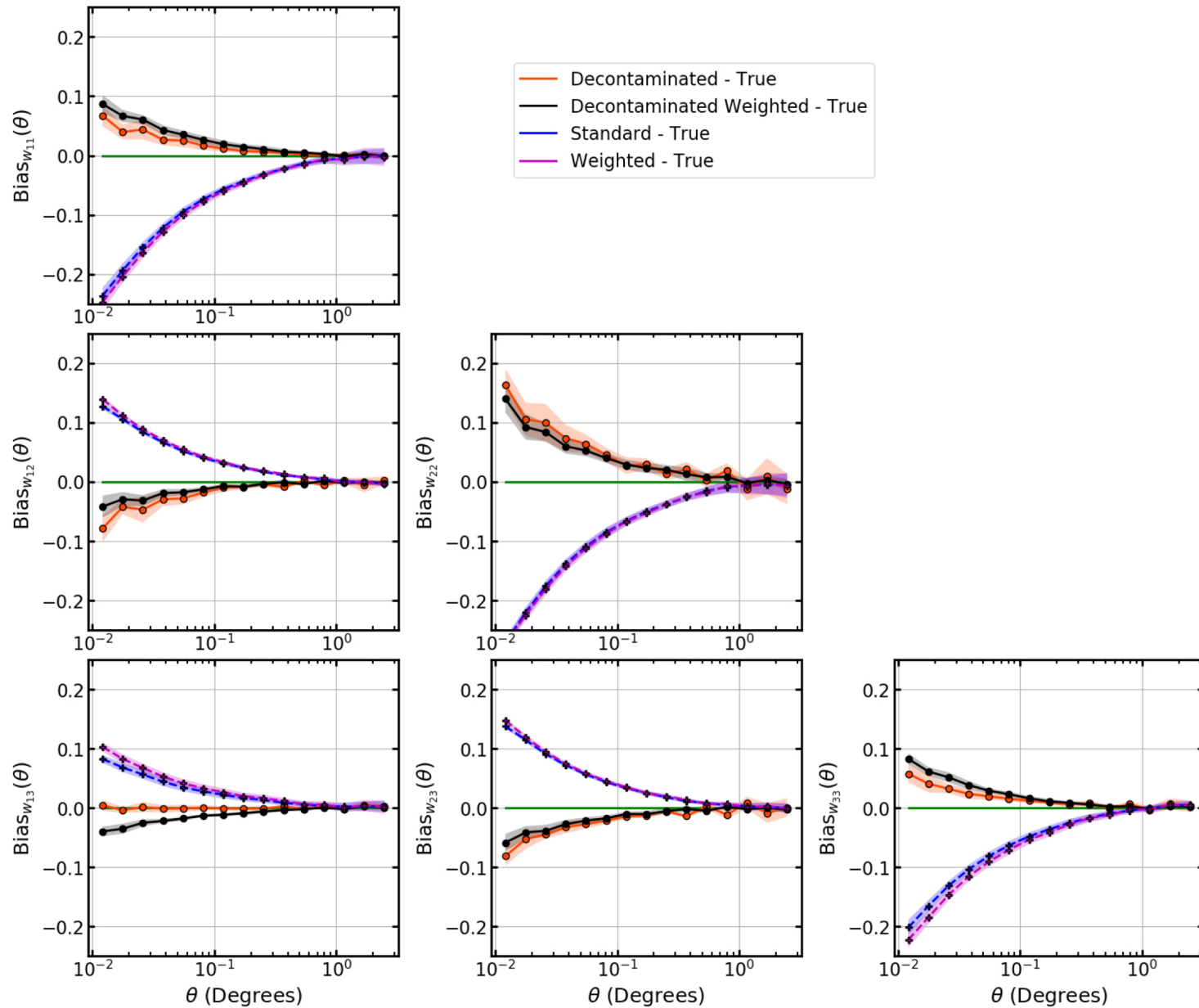
Figure 15. from Angular Correlation Function Estimators Accounting for Contamination from Probabilistic Distance Measurements null 2020 APJ 890 78 doi:10.3847/1538-4357/ab63c8 https://dx.doi.org/10.3847/1538-4357/ab63c8 © 2020. The American Astronomical Society. All rights reserved.
