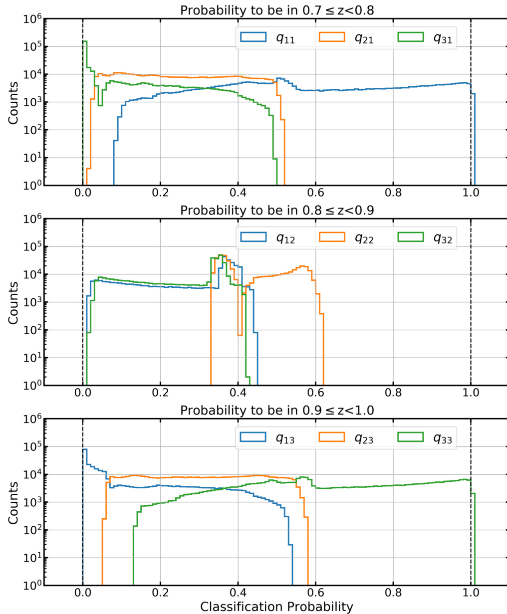
Figure 14. from Angular Correlation Function Estimators Accounting for Contamination from Probabilistic Distance Measurements null 2020 APJ 890 78 doi:10.3847/1538-4357/ab63c8 https://dx.doi.org/10.3847/1538-4357/ab63c8 © 2020. The American Astronomical Society. All rights reserved.
