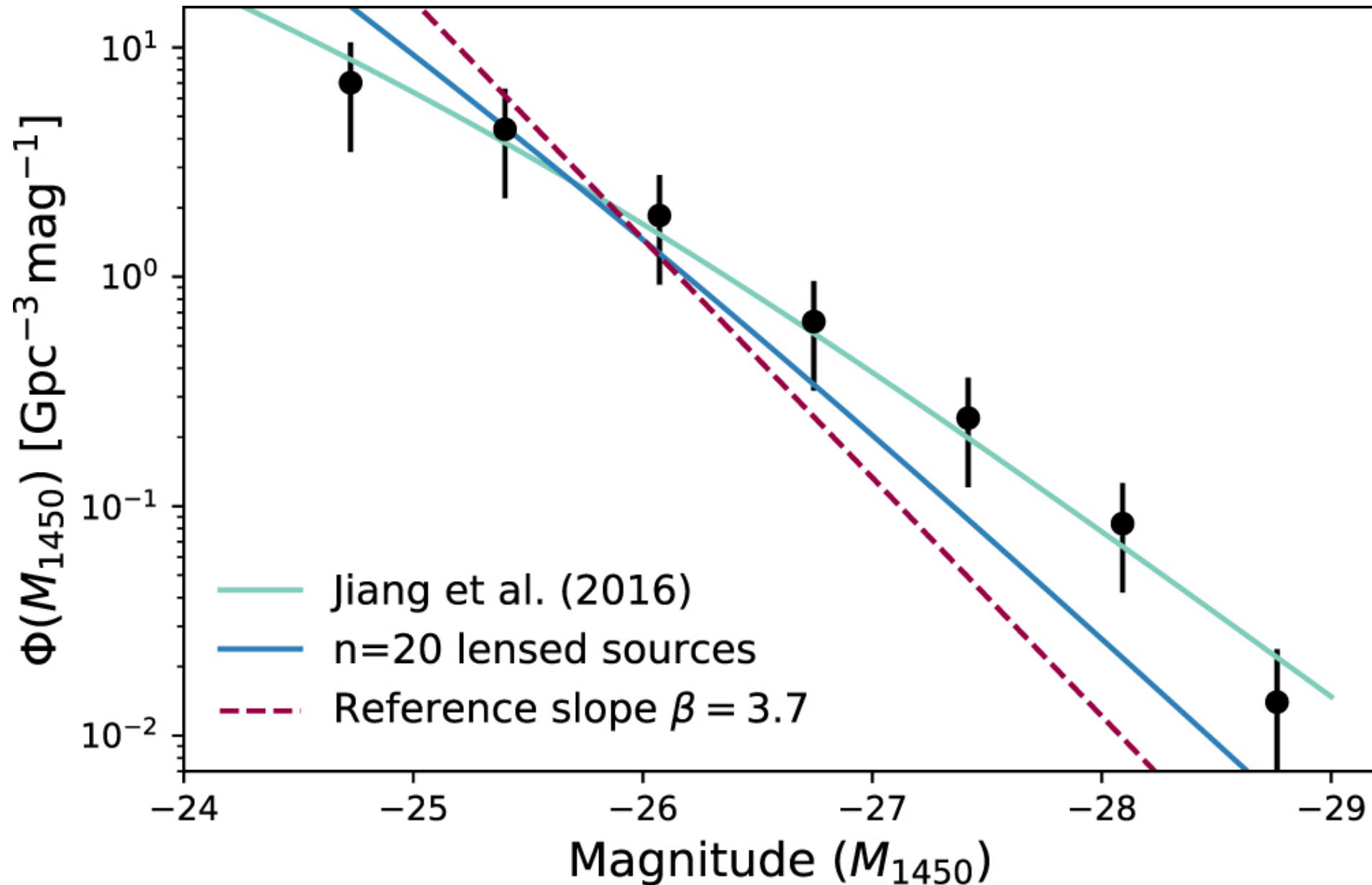
Figure 4. from Reality or Mirage? Observational Test and Implications for the Claimed Extremely Magnified Quasar at z = 6.3 null 2020 APJ 889 52 doi:10.3847/1538-4357/ab6130 https://dx.doi.org/10.3847/1538-4357/ab6130 © 2020. The American Astronomical Society. All rights reserved.
