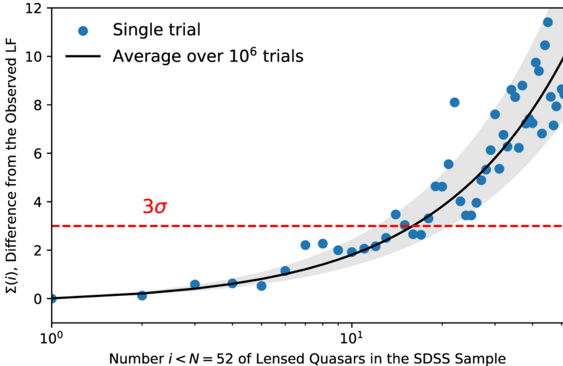
Figure 3. from Reality or Mirage? Observational Test and Implications for the Claimed Extremely Magnified Quasar at z = 6.3 null 2020 APJ 889 52 doi:10.3847/1538-4357/ab6130 https://dx.doi.org/10.3847/1538-4357/ab6130 © 2020. The American Astronomical Society. All rights reserved.
