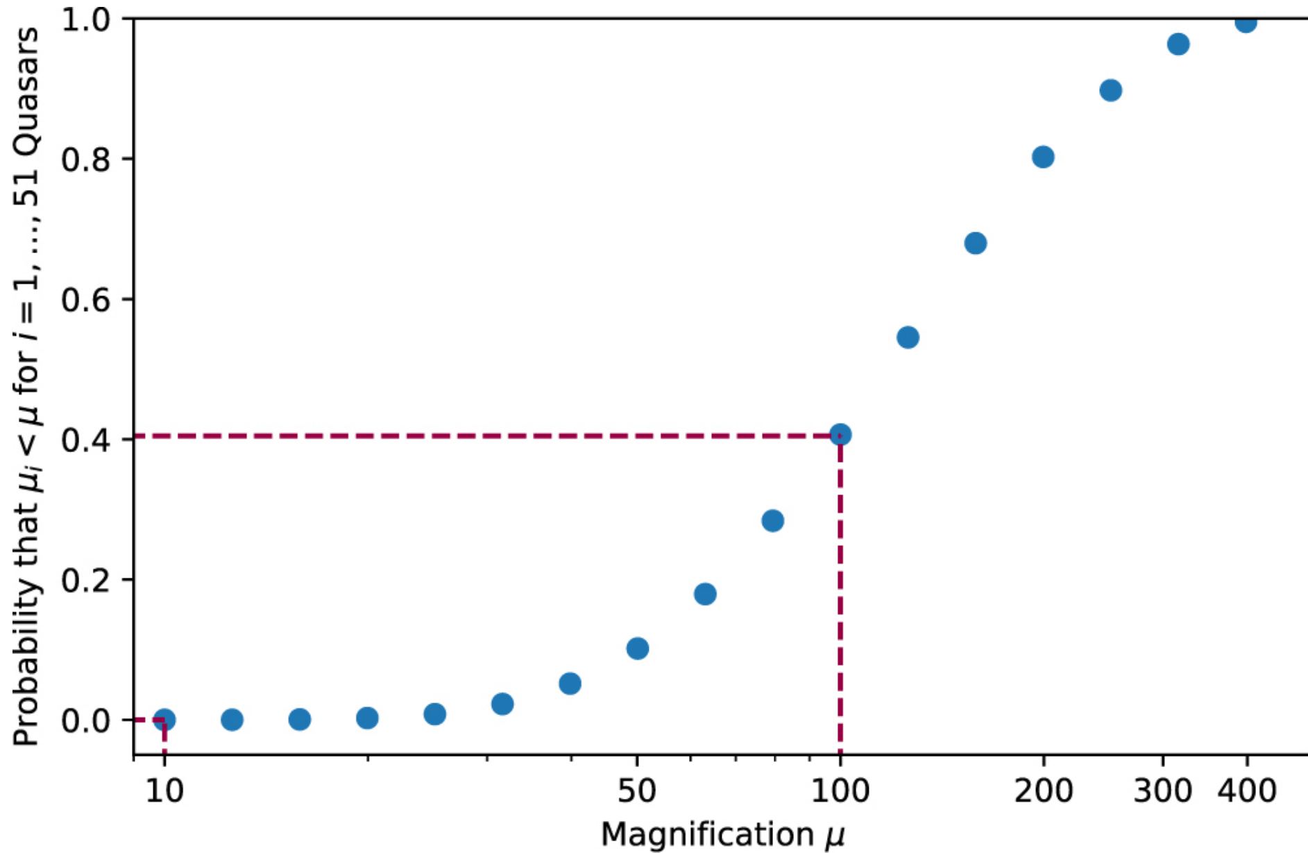
Figure 2. from Reality or Mirage? Observational Test and Implications for the Claimed Extremely Magnified Quasar at z = 6.3 null 2020 APJ 889 52 doi:10.3847/1538-4357/ab6130 https://dx.doi.org/10.3847/1538-4357/ab6130 © 2020. The American Astronomical Society. All rights reserved.
