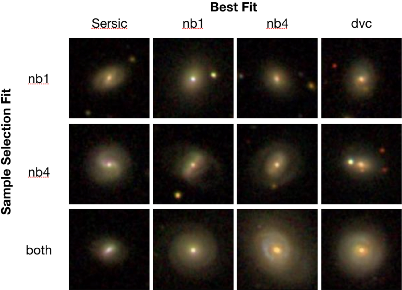
Figure 7. from BreakBRD Galaxies. I. Global Properties of Spiral Galaxies with Central Star Formation in Red Disks null 2020 APJ 889 188 doi:10.3847/1538-4357/ab5dbb https://dx.doi.org/10.3847/1538-4357/ab5dbb © 2020. The American Astronomical Society.
