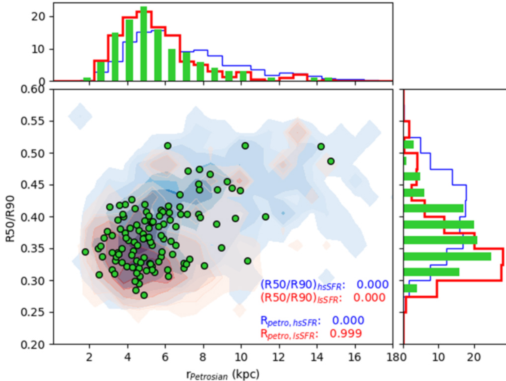
Figure 5. from BreakBRD Galaxies. I. Global Properties of Spiral Galaxies with Central Star Formation in Red Disks null 2020 APJ 889 188 doi:10.3847/1538-4357/ab5dbb https://dx.doi.org/10.3847/1538-4357/ab5dbb © 2020. The American Astronomical Society.
