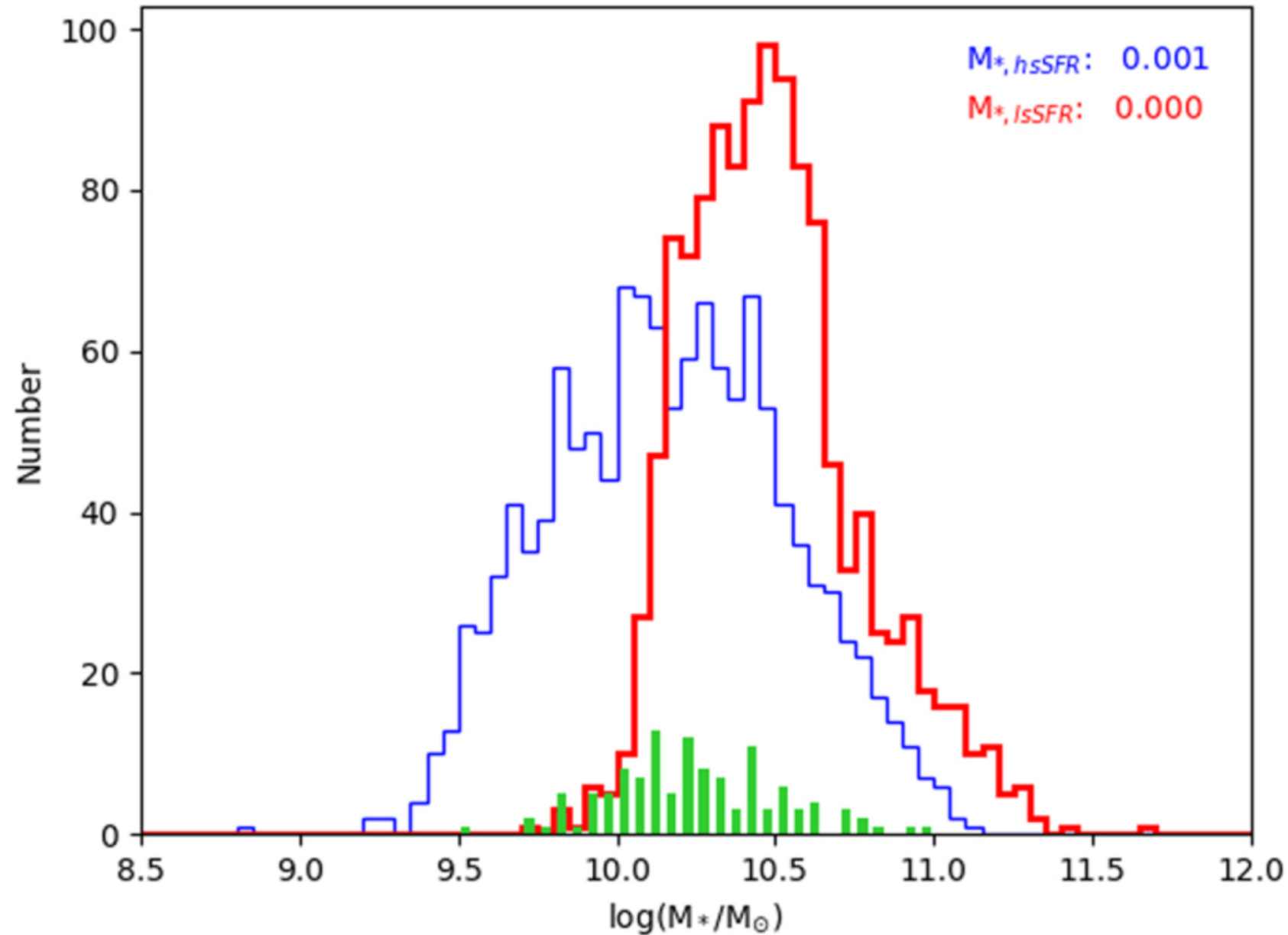
Figure 3. from BreakBRD Galaxies. I. Global Properties of Spiral Galaxies with Central Star Formation in Red Disks null 2020 APJ 889 188 doi:10.3847/1538-4357/ab5dbb https://dx.doi.org/10.3847/1538-4357/ab5dbb © 2020. The American Astronomical Society.
