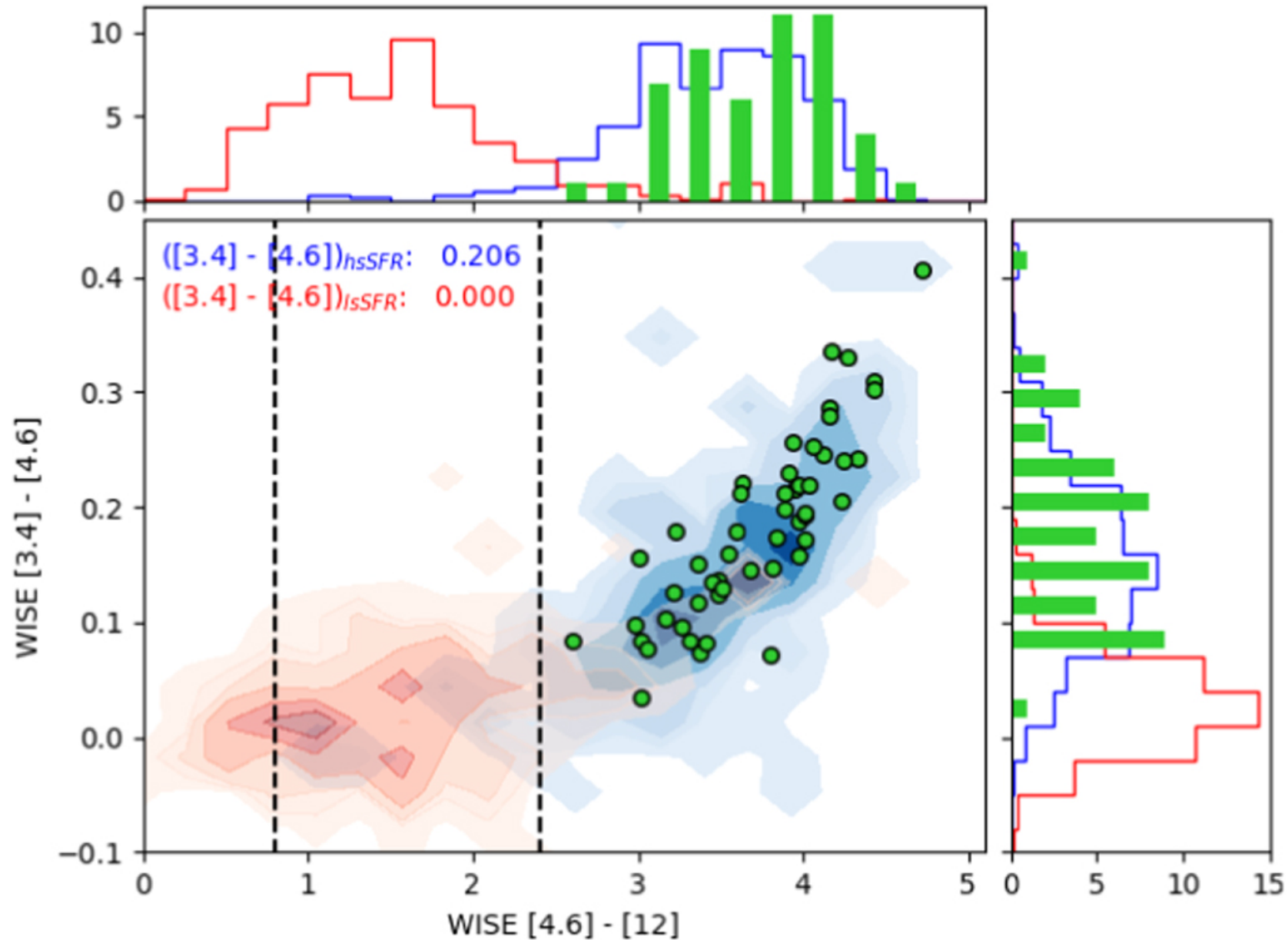
Figure 12. from BreakBRD Galaxies. I. Global Properties of Spiral Galaxies with Central Star Formation in Red Disks null 2020 APJ 889 188 doi:10.3847/1538-4357/ab5dbb https://dx.doi.org/10.3847/1538-4357/ab5dbb © 2020. The American Astronomical Society.
