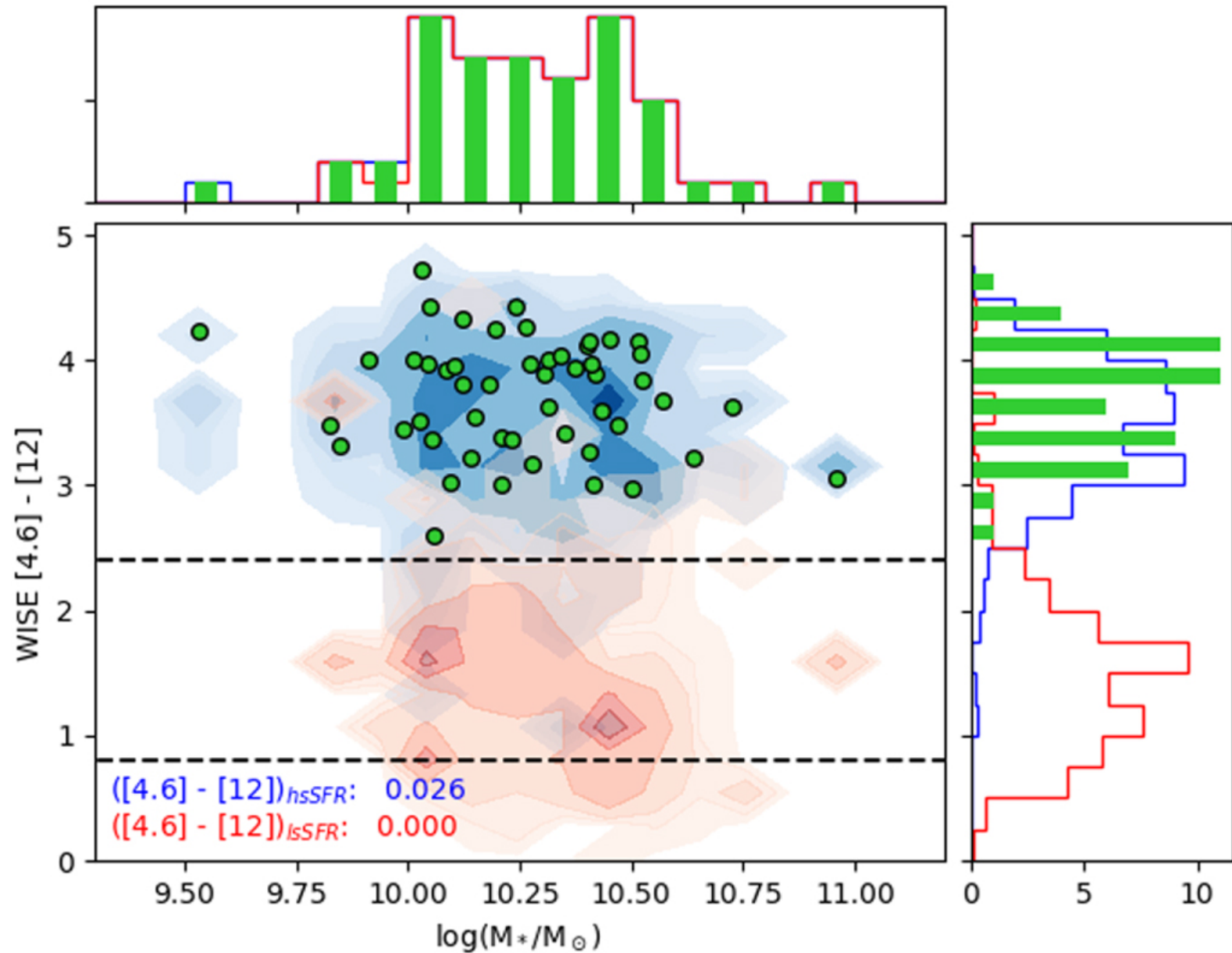
Figure 11. from BreakBRD Galaxies. I. Global Properties of Spiral Galaxies with Central Star Formation in Red Disks null 2020 APJ 889 188 doi:10.3847/1538-4357/ab5dbb https://dx.doi.org/10.3847/1538-4357/ab5dbb © 2020. The American Astronomical Society.
