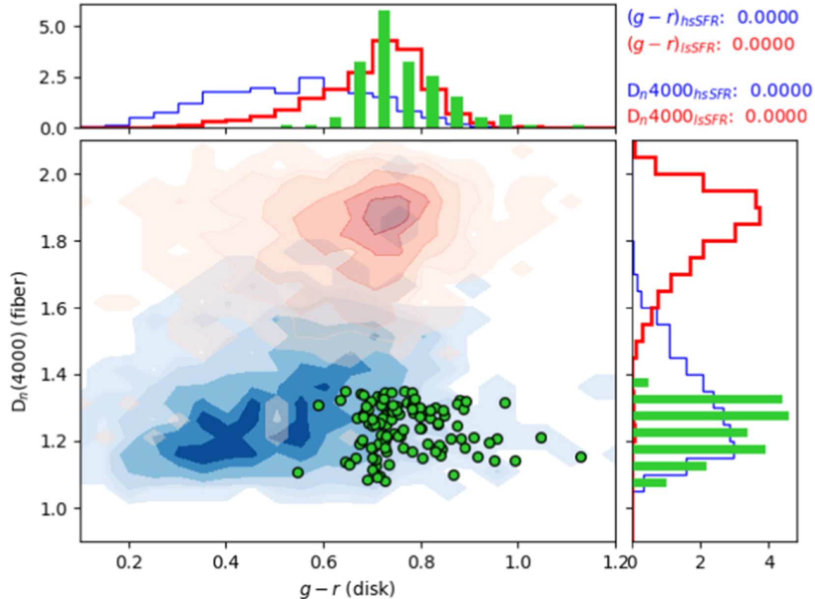
Figure 1. from BreakBRD Galaxies. I. Global Properties of Spiral Galaxies with Central Star Formation in Red Disks null 2020 APJ 889 188 doi:10.3847/1538-4357/ab5dbb https://dx.doi.org/10.3847/1538-4357/ab5dbb © 2020. The American Astronomical Society.
