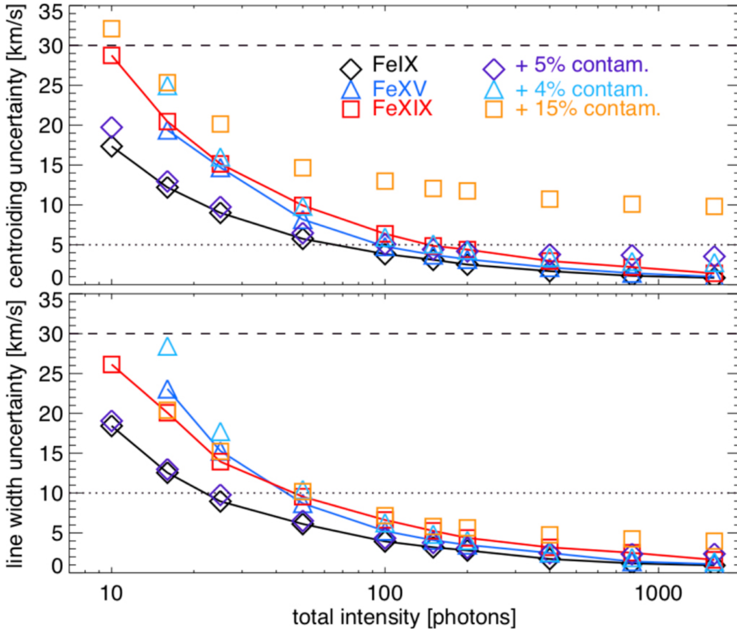
Figure 6. from The Multi-slit Approach to Coronal Spectroscopy with the Multi-slit Solar Explorer (MUSE) null 2020 APJ 888 3 doi:10.3847/1538-4357/ab5b03 https://dx.doi.org/10.3847/1538-4357/ab5b03 © 2019. The American Astronomical Society.
