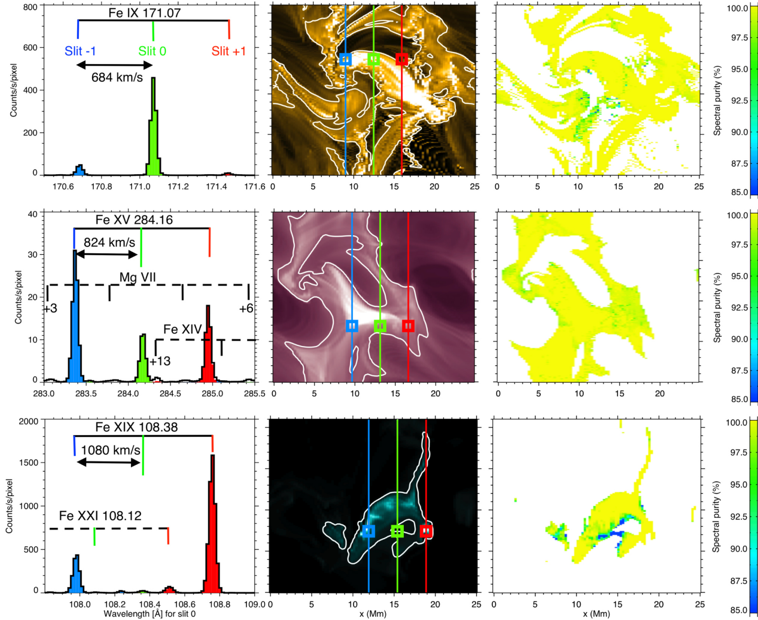
Figure 5. from The Multi-slit Approach to Coronal Spectroscopy with the Multi-slit Solar Explorer (MUSE) null 2020 APJ 888 3 doi:10.3847/1538-4357/ab5b03 https://dx.doi.org/10.3847/1538-4357/ab5b03 © 2019. The American Astronomical Society.
